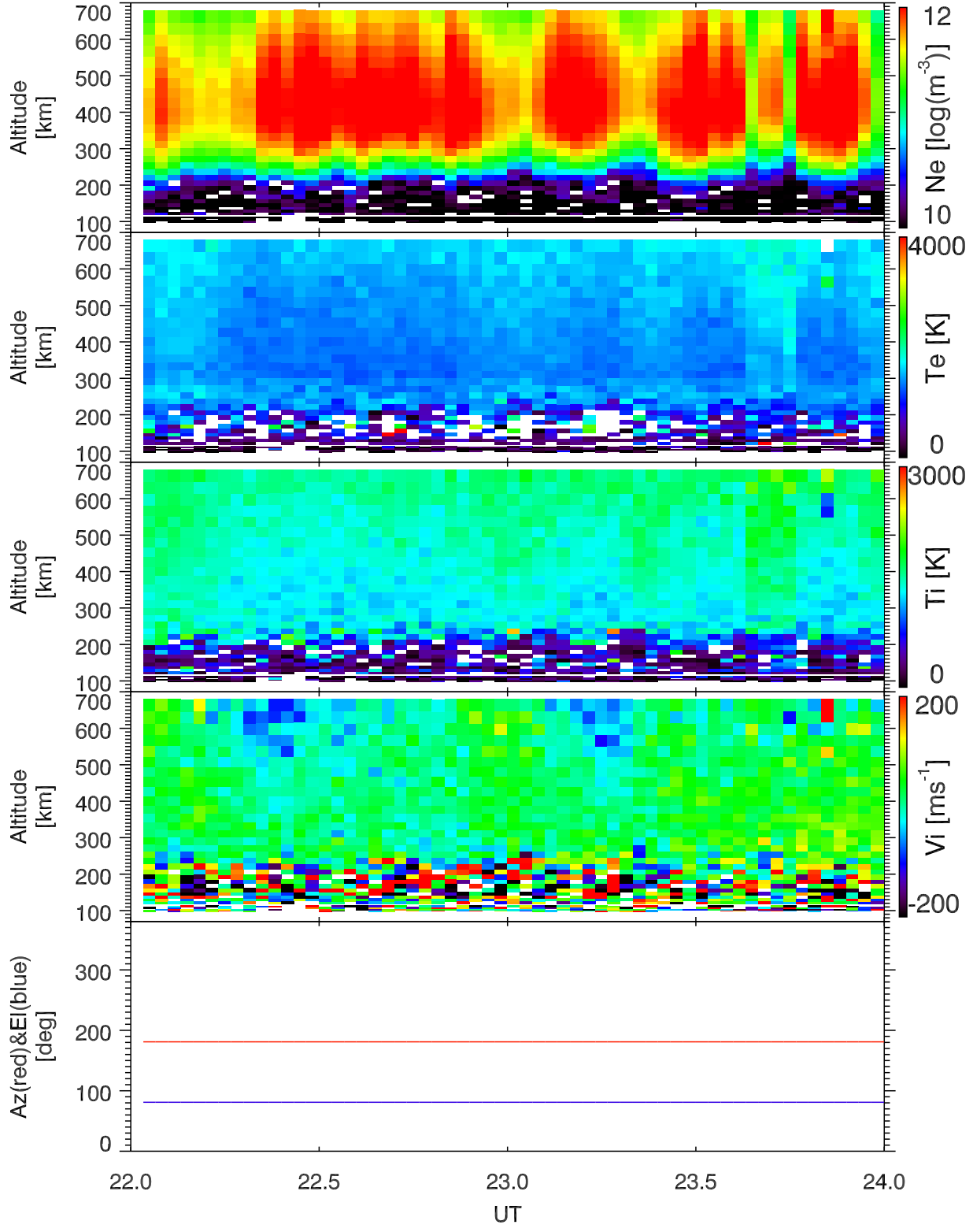
EISCAT 2001-10-16_22_24UT_tau0_120@42m.
