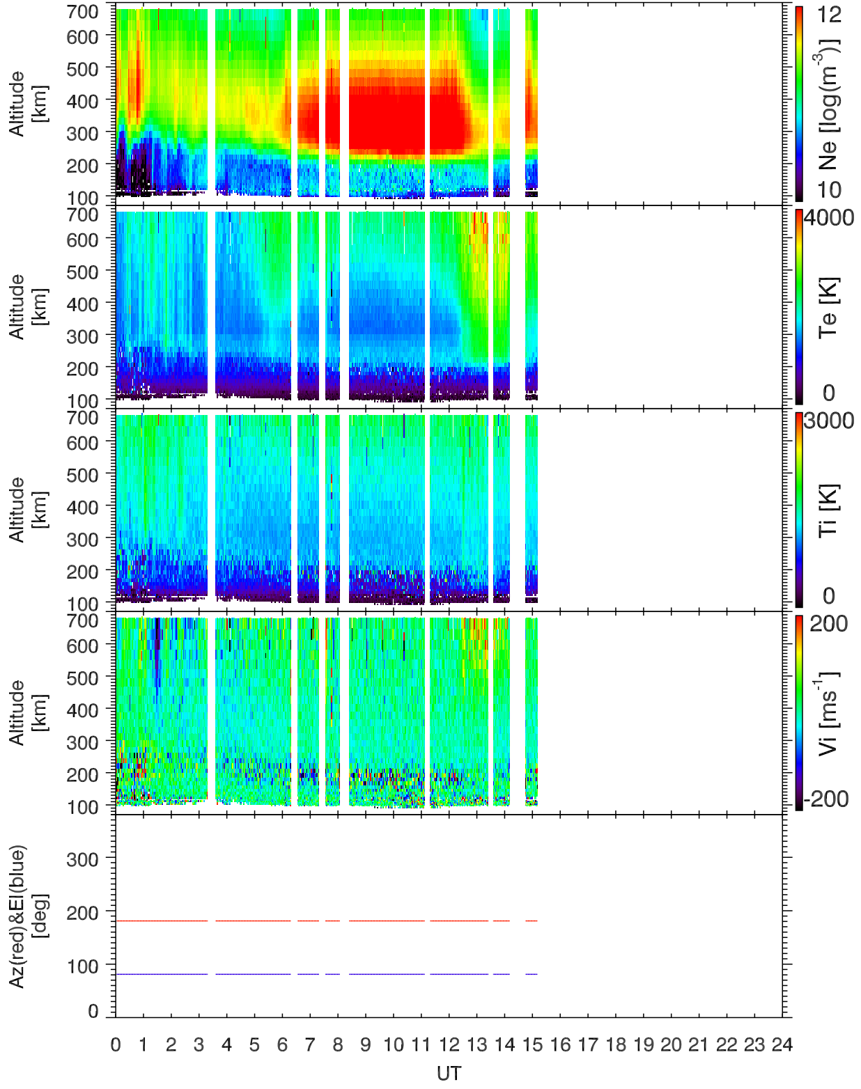
EISCAT 2001-10-18_00_24UT_tau0_120@42m.
