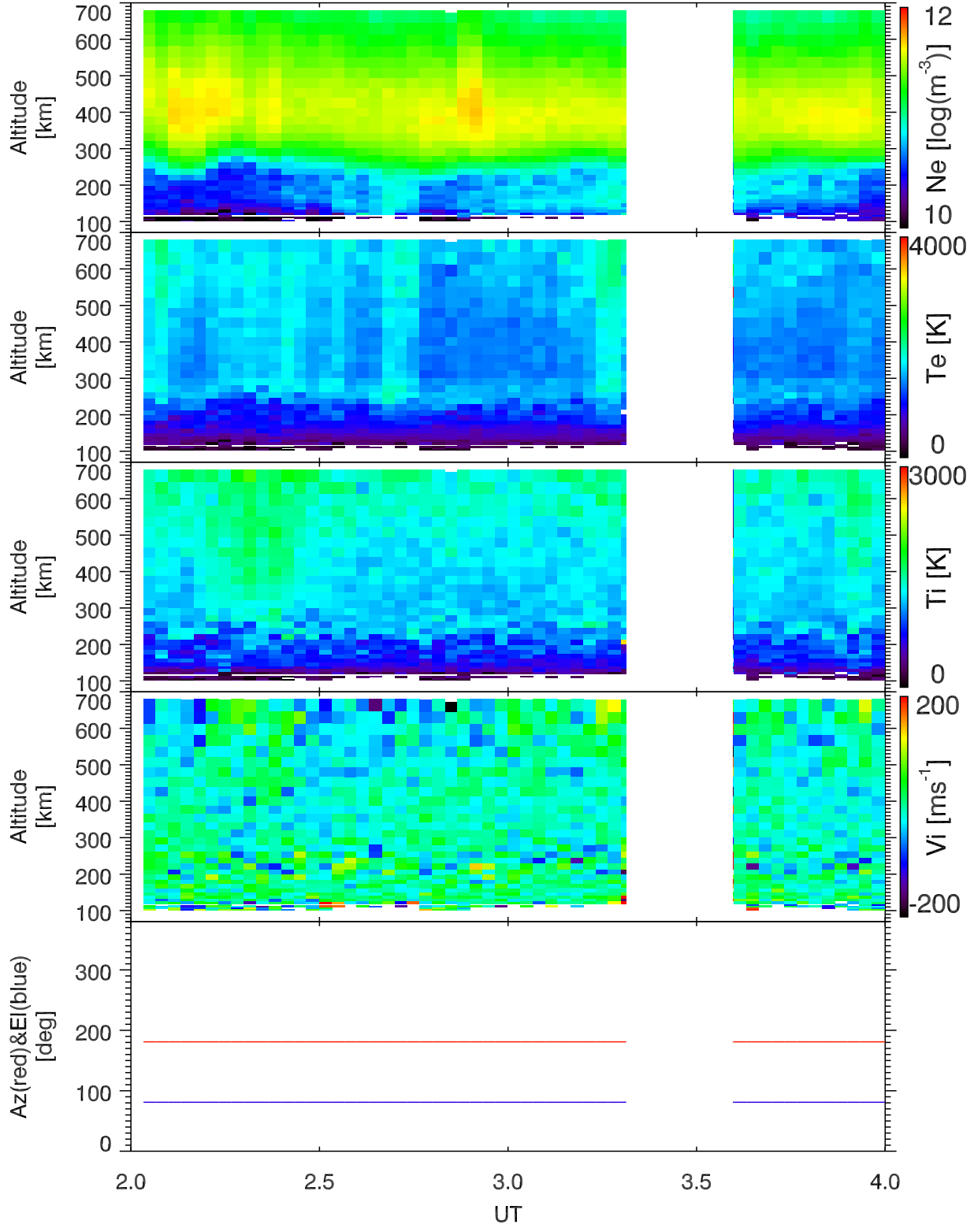
EISCAT 2001-10-18_02_04UT_tau0_120@42m.
