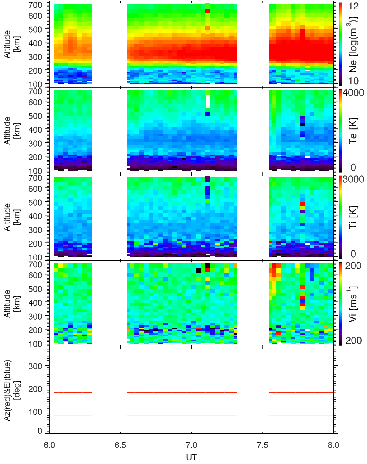
EISCAT 2001-10-18_06_08UT_tau0_120@42m.
