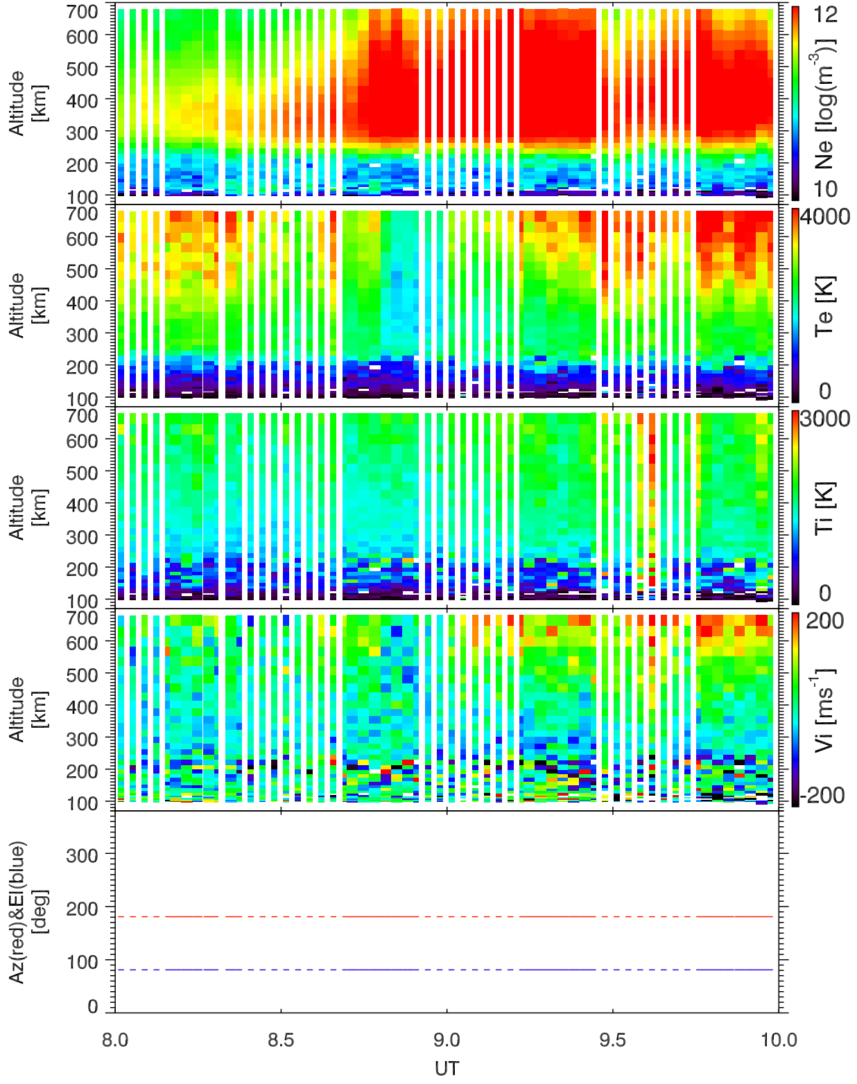
EISCAT 2001-10-20_08_10UT_tau0_120@42m.
