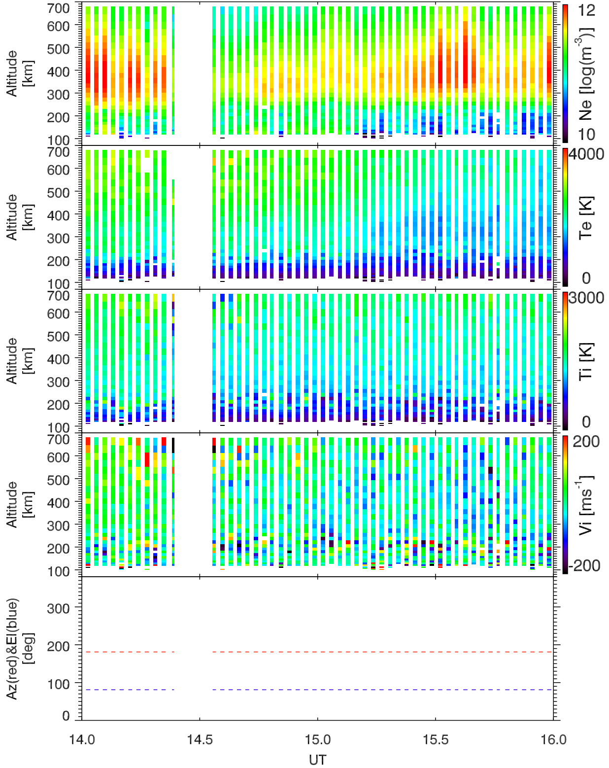
EISCAT 2001-10-27_14_16UT_tau0_ant@42m.
