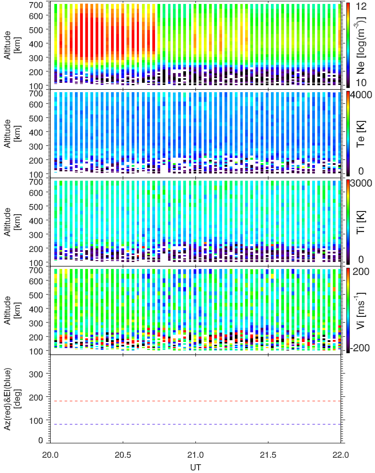
EISCAT 2001-10-27_20_22UT_tau0_ant@42m.
