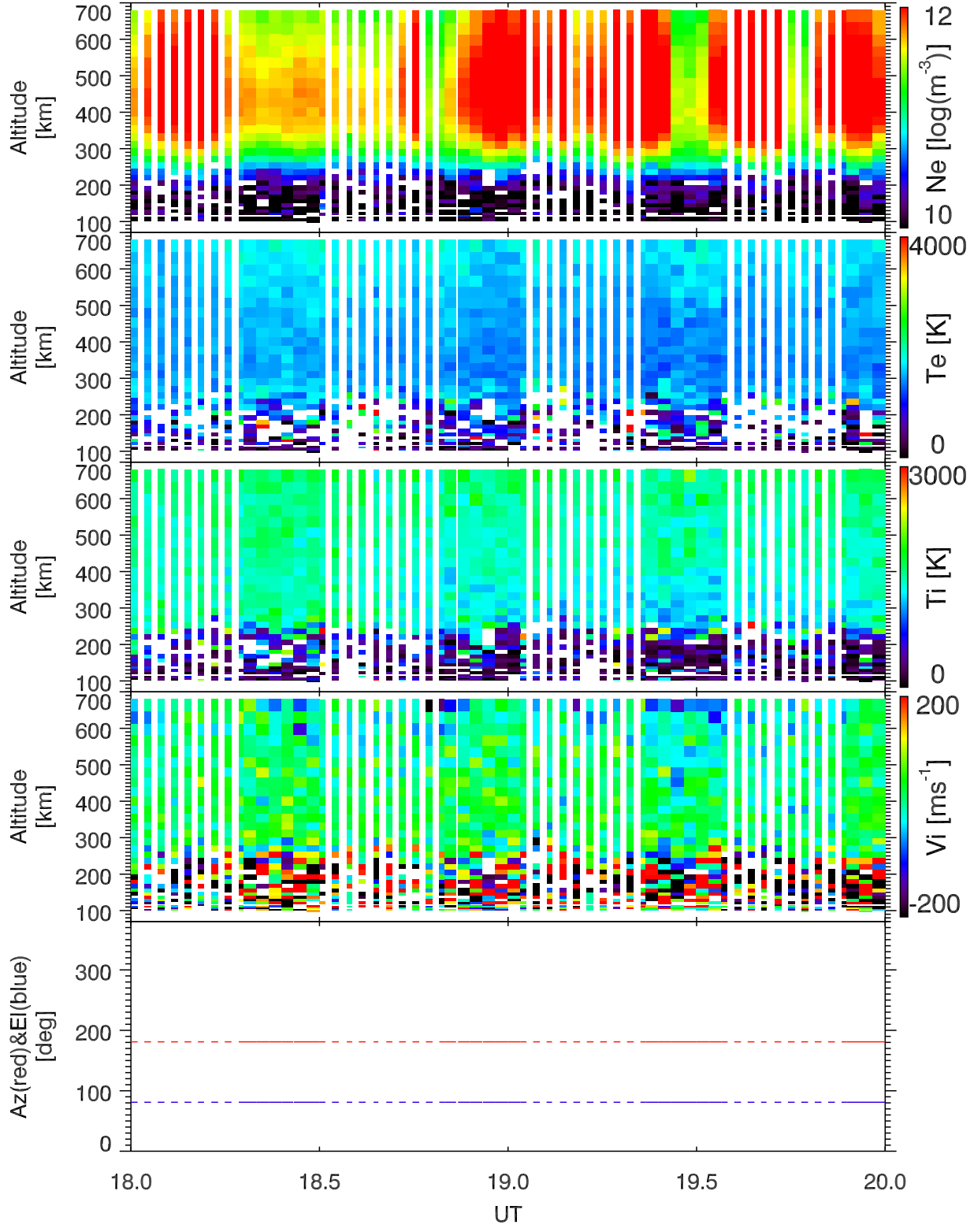
EISCAT 2001-10-29_18_20UT_tau0_120@42m.
