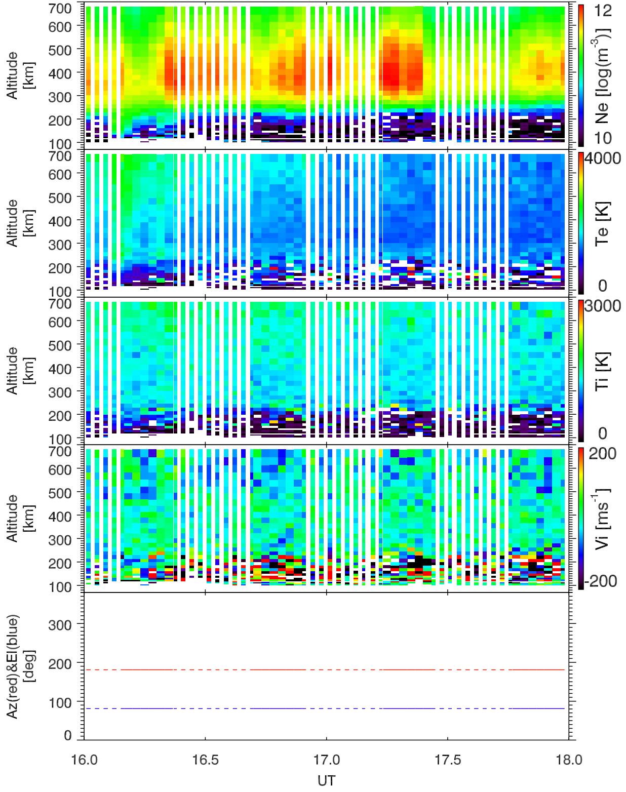
EISCAT 2001-10-30_16_18UT_tau0_120@42m.
