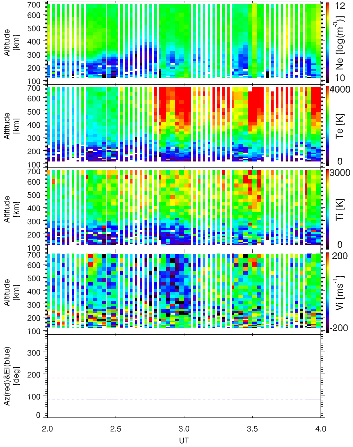
EISCAT 2001-11-06_02_04UT_tau0_120@42m.
