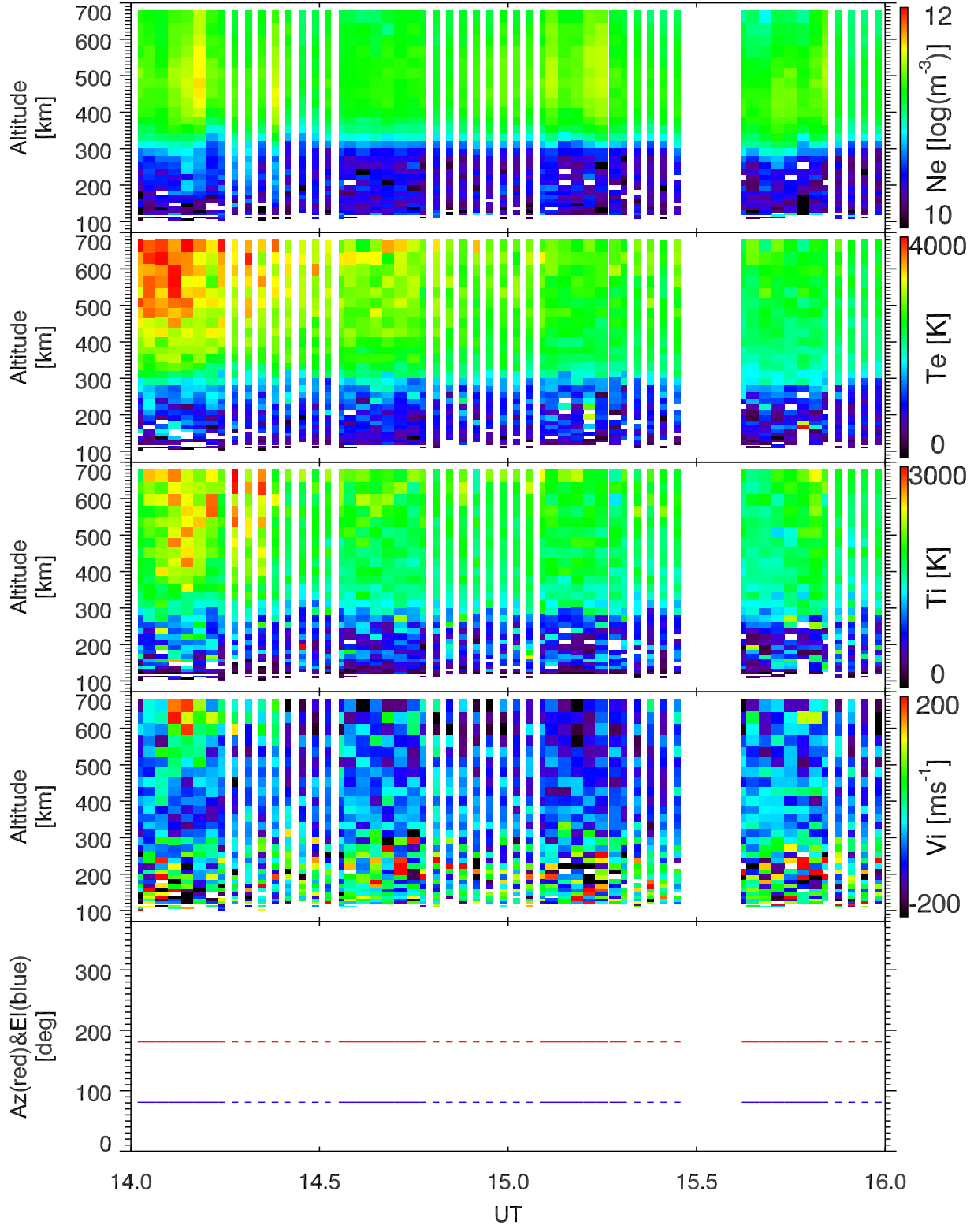
EISCAT 2001-11-06_14_16UT_tau0_120@42m.
