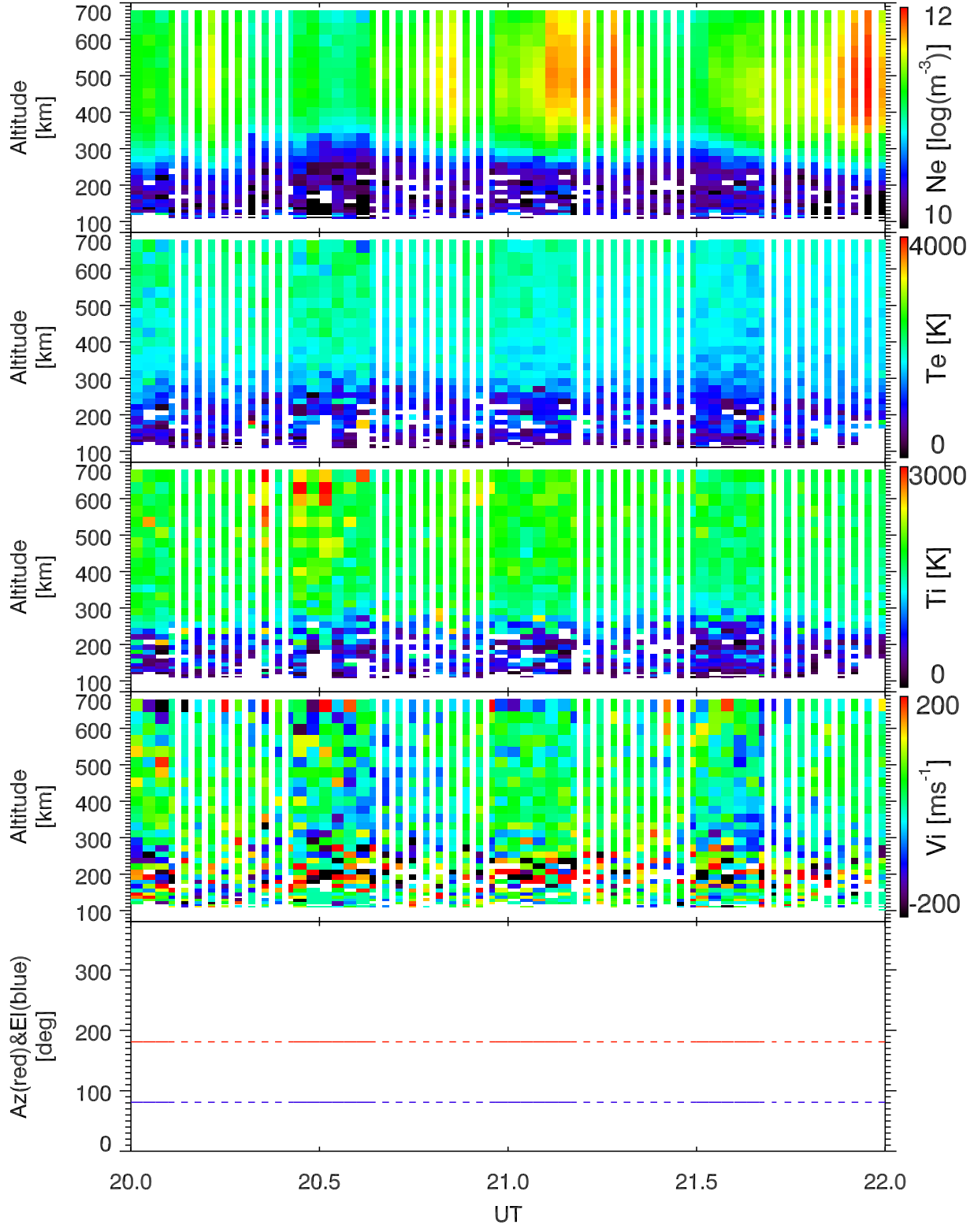
EISCAT 2001-11-06_20_22UT_tau0_120@42m.
