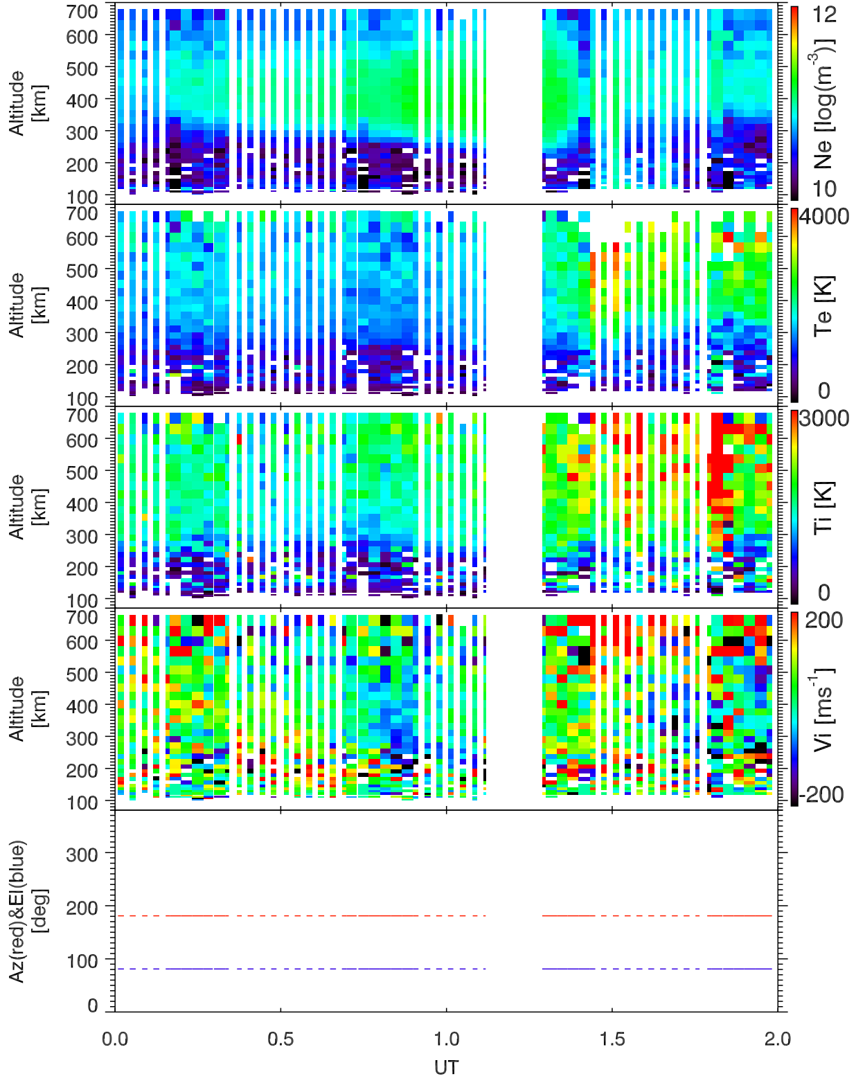
EISCAT 2001-11-07_00_02UT_tau0_120@42m.
