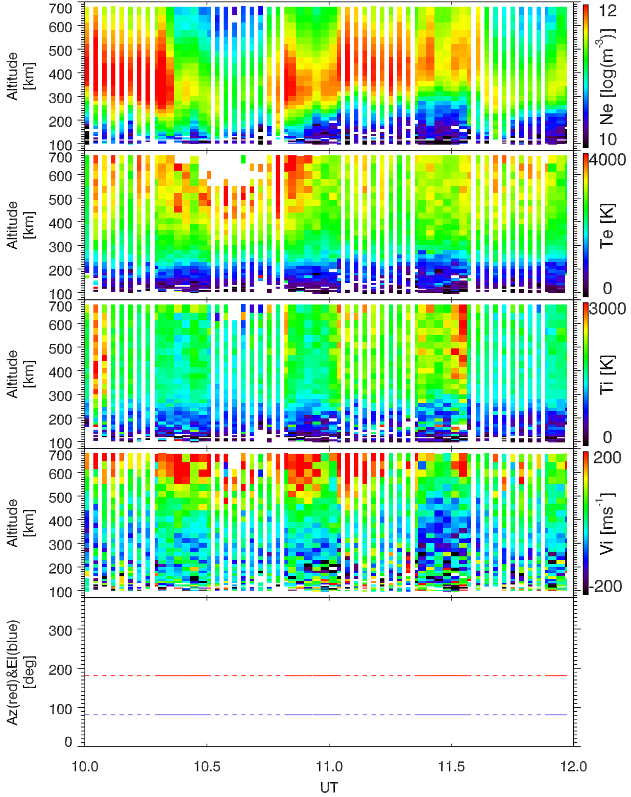
EISCAT 2001-11-07_10_12UT_tau0_120@42m.
