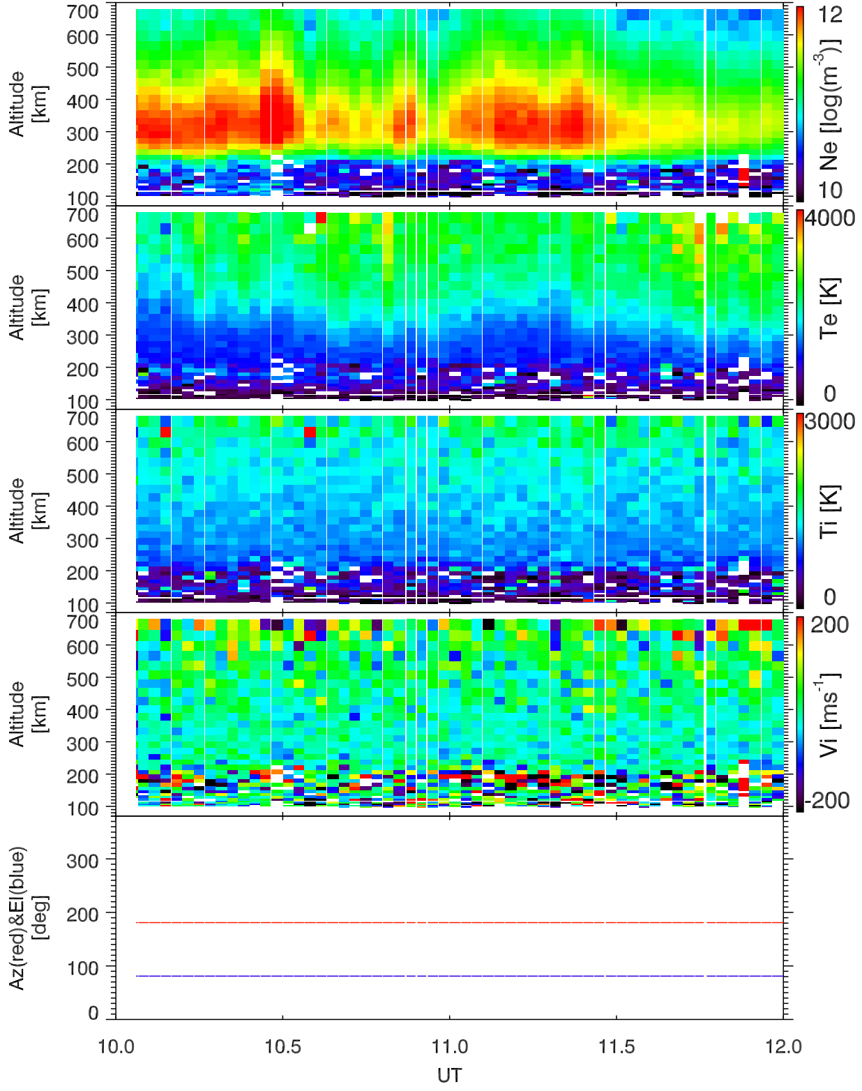
EISCAT 2001-11-13_10_12UT_tau0_120@42m.
