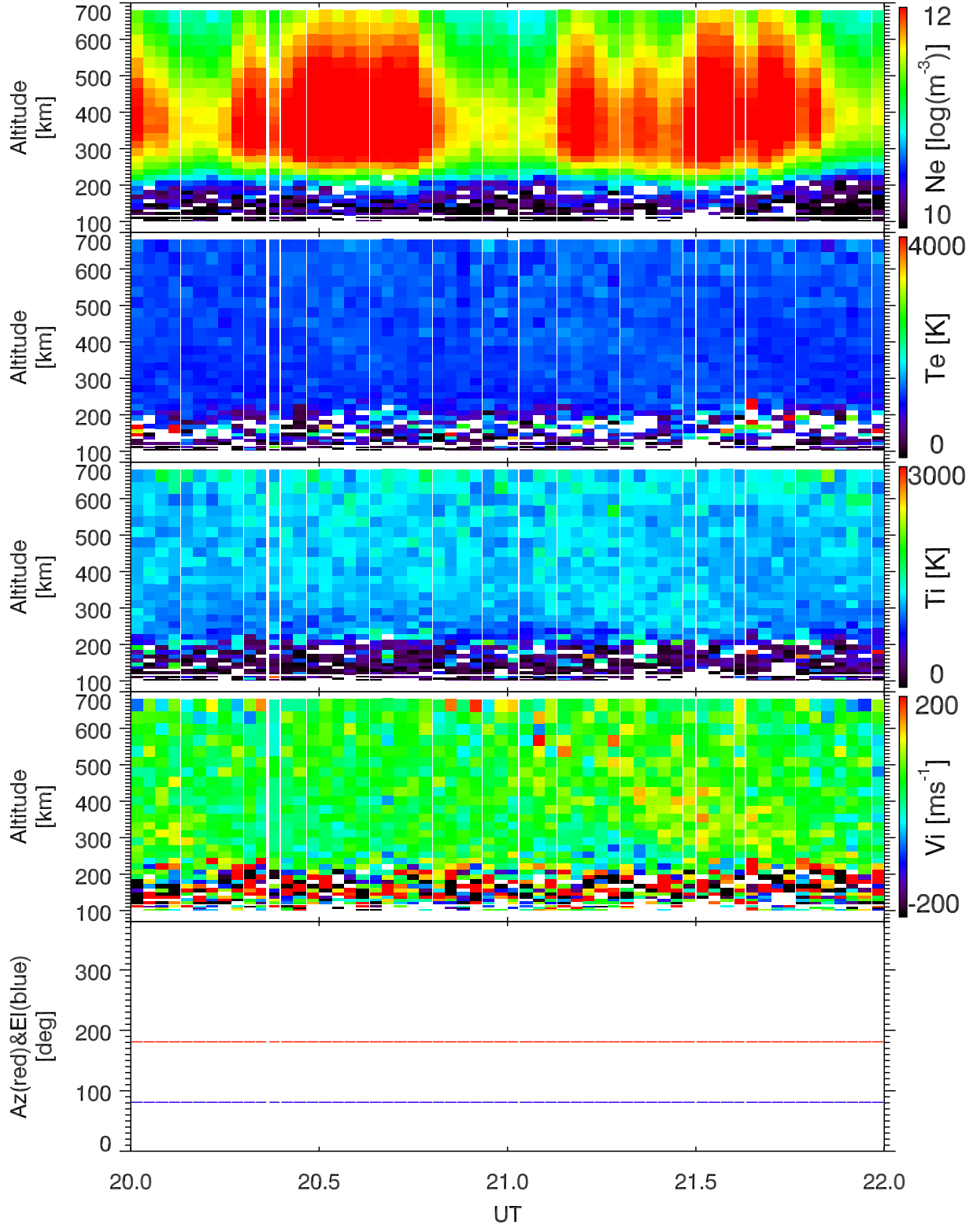
EISCAT 2001-11-13_20_22UT_tau0_120@42m.
