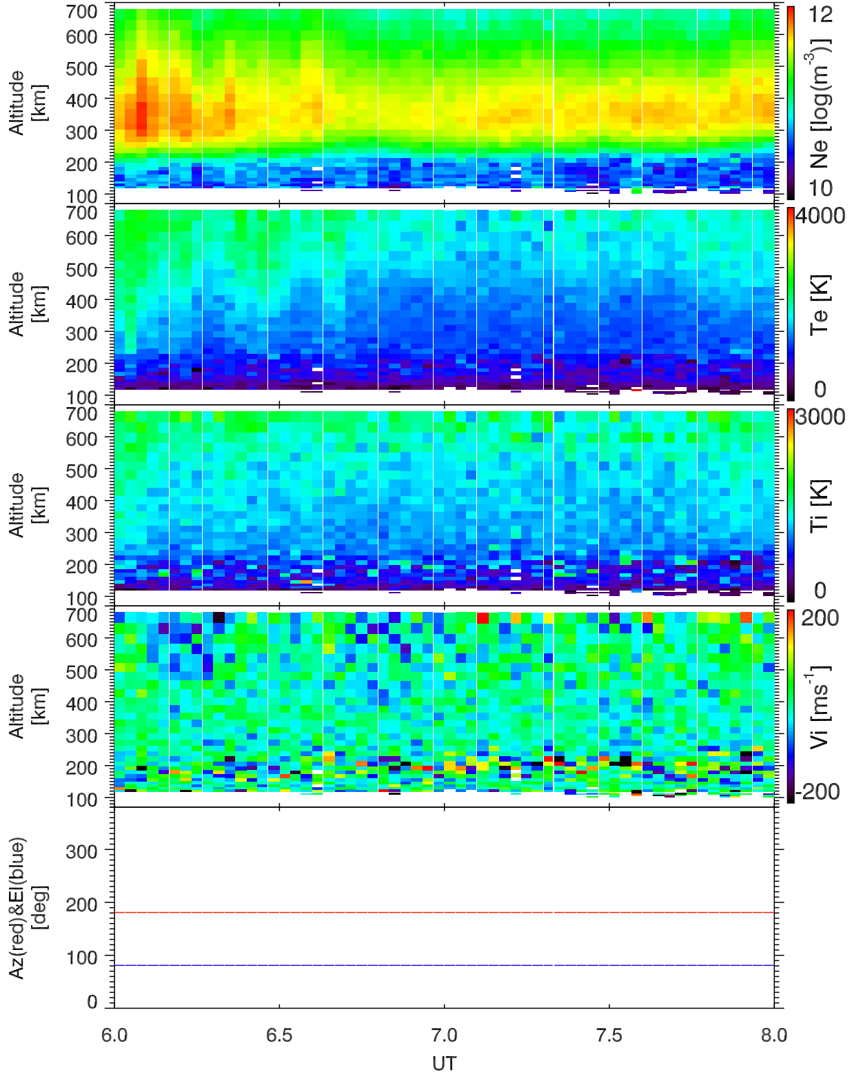
EISCAT 2001-11-14_06_08UT_tau0_120@42m.
