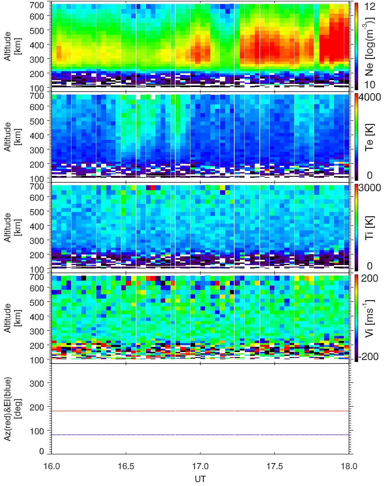
EISCAT 2001-11-14_16_18UT_tau0_120@42m.
