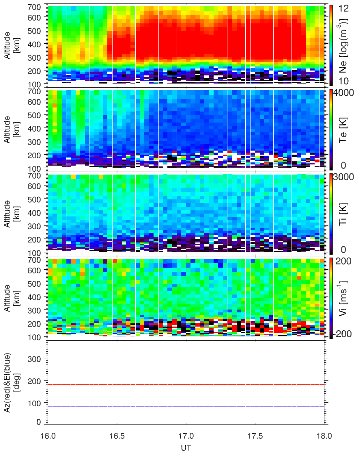
EISCAT 2001-11-15_16_18UT_tau0_all@42m.
