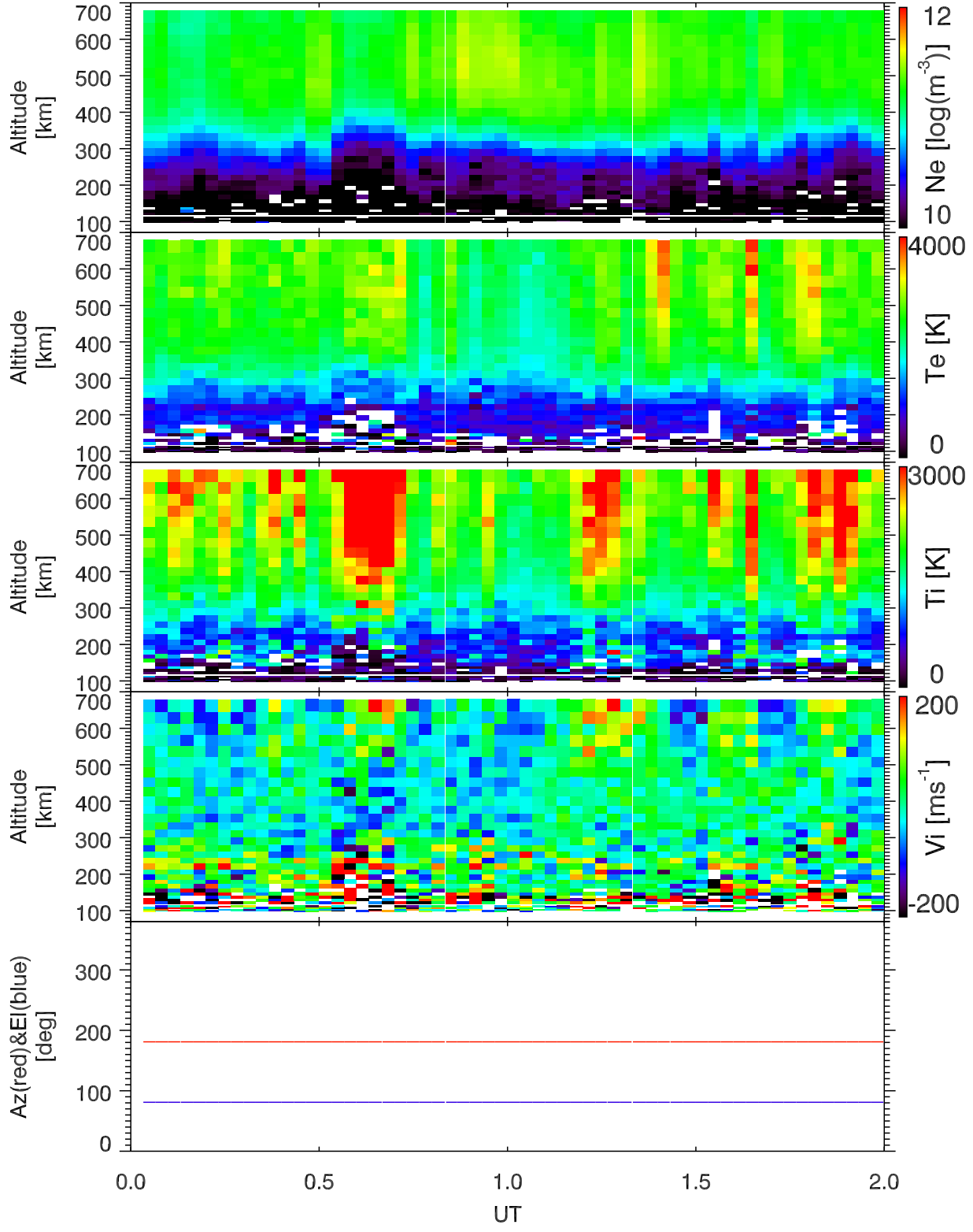
EISCAT 2001-11-16_00_02UT_tau0_120@42m.
