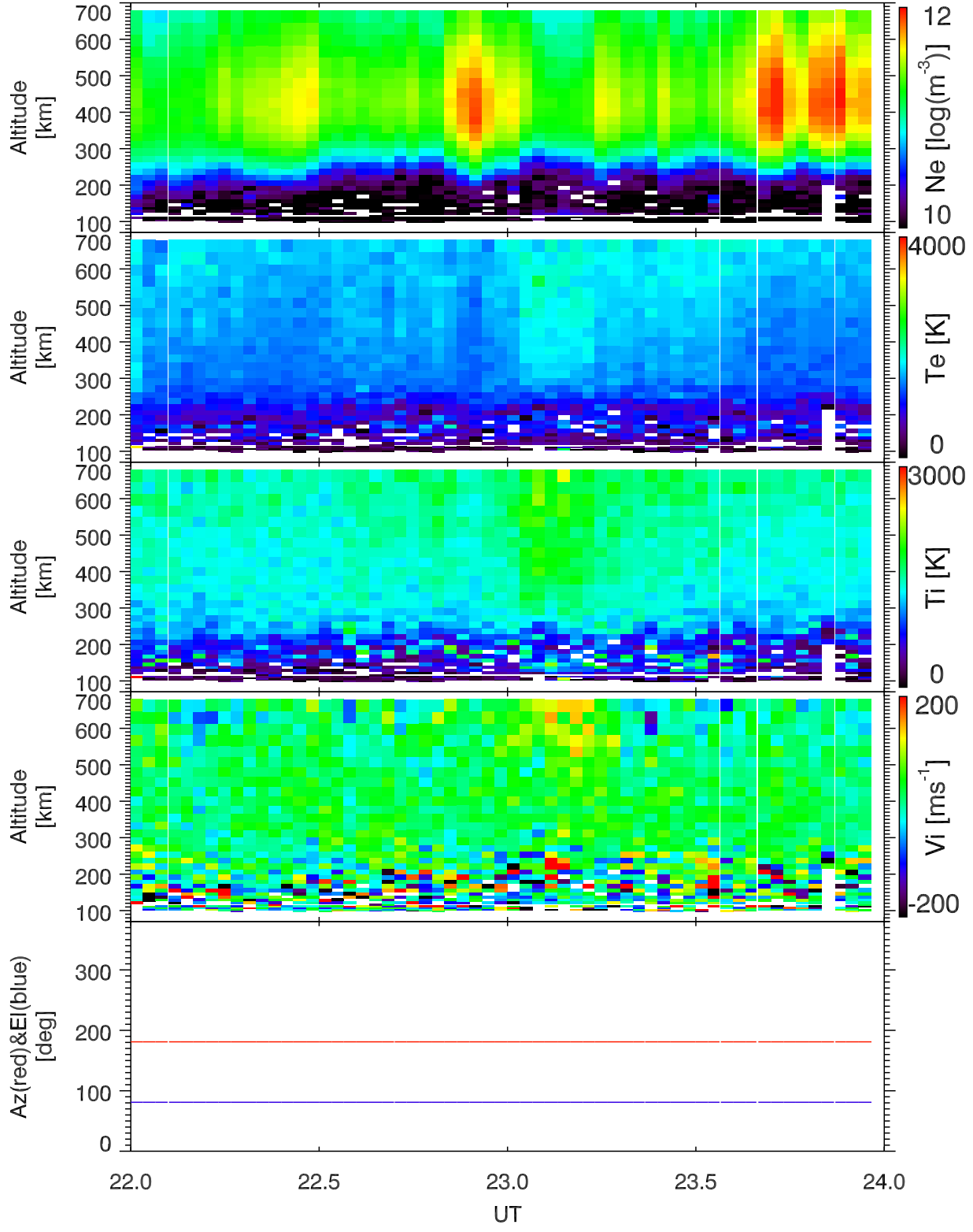
EISCAT 2001-11-17_22_24UT_tau0_120@42m.
