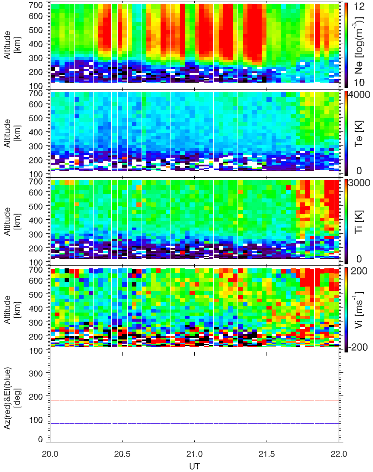
EISCAT 2001-11-19_20_22UT_tau0_all@42m.
