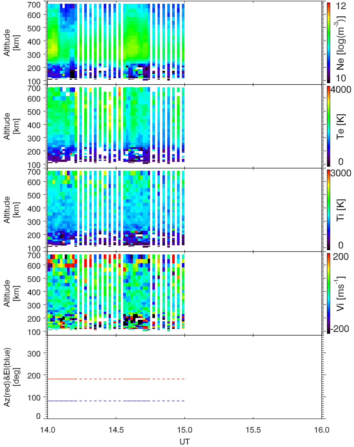
EISCAT 2001-11-20_14_16UT_tau0_all@42m.
