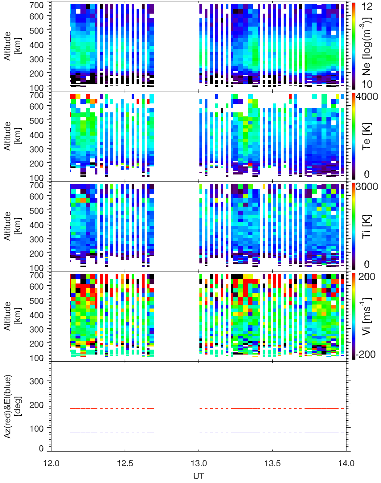
EISCAT 2001-11-27_12_14UT_tau0_120@42m.
