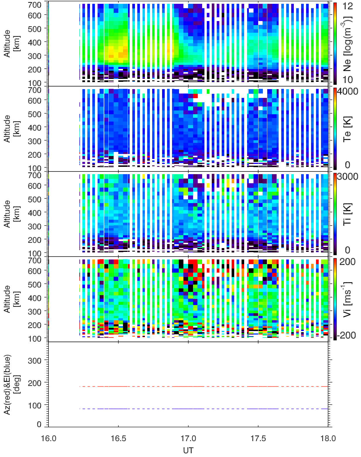
EISCAT 2001-12-11_16_18UT_tau0_120@42m.
