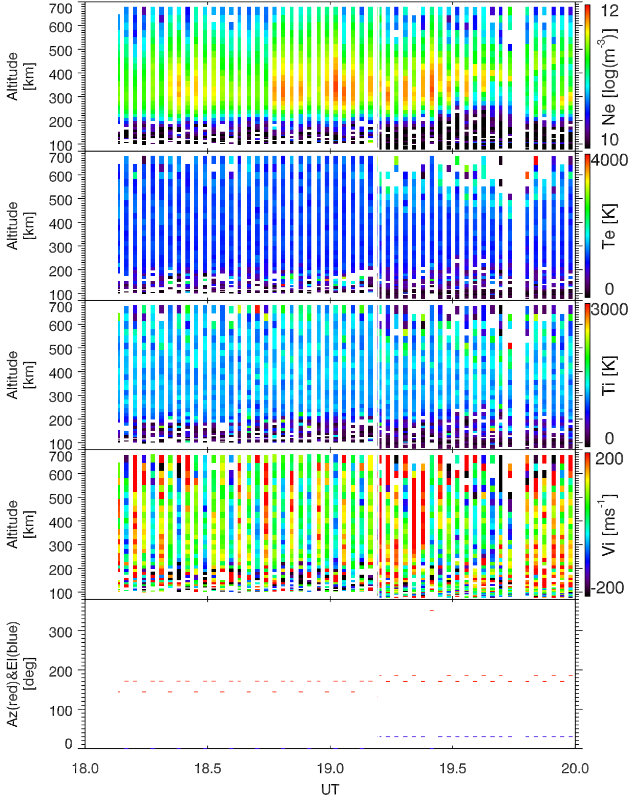
EISCAT 2001-12-11_18_20UT_tau0_ant@32m.
