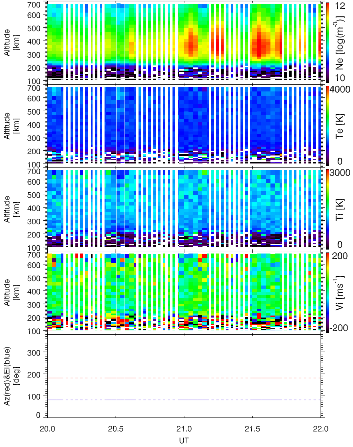
EISCAT 2001-12-11_20_22UT_tau0_120@42m.
