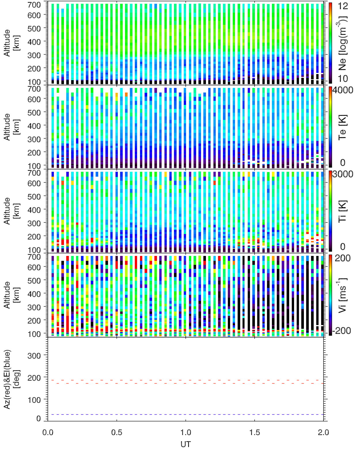
EISCAT 2001-12-12_00_02UT_tau0_ant@32m.
