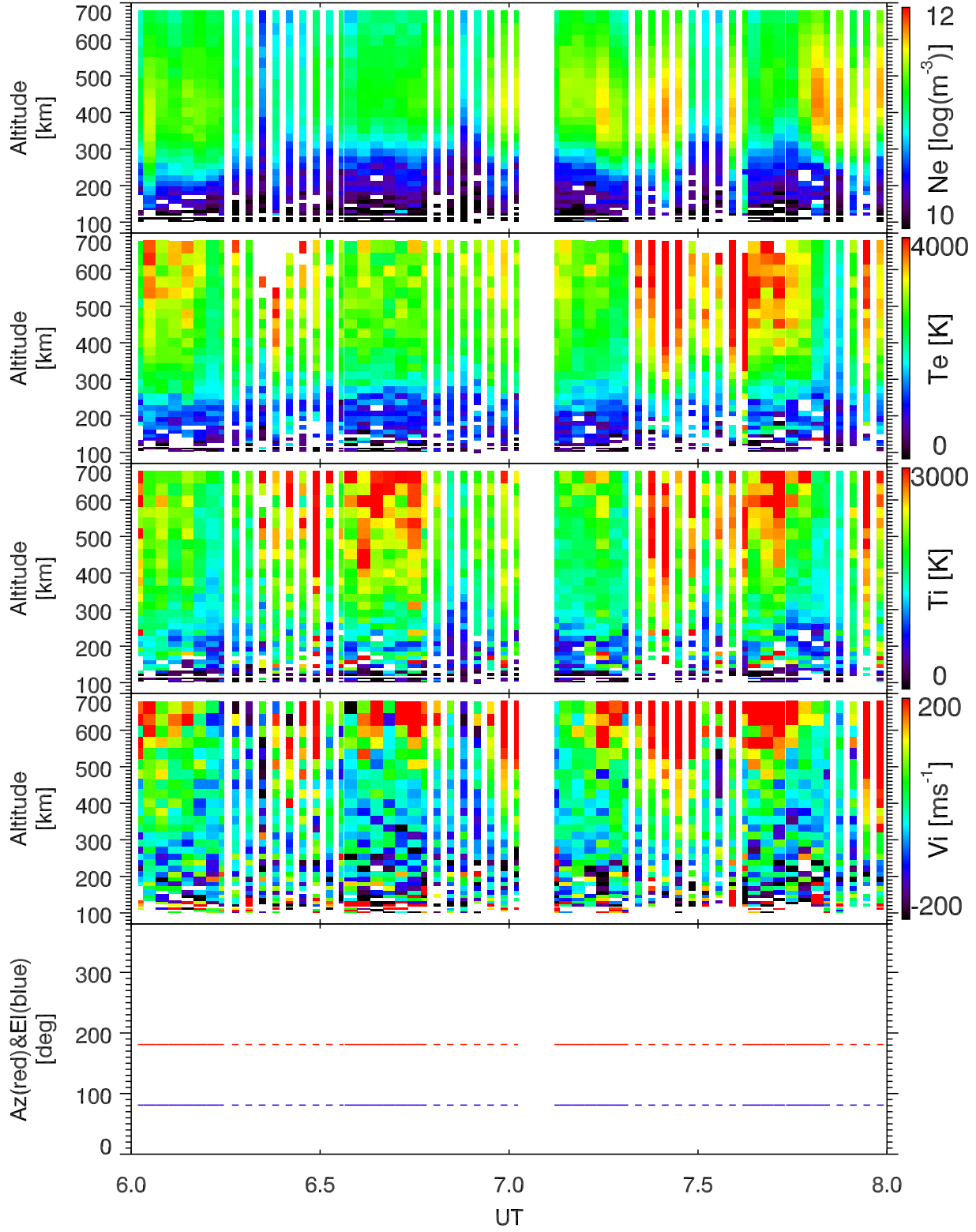
EISCAT 2001-12-12_06_08UT_tau0_120@42m.
