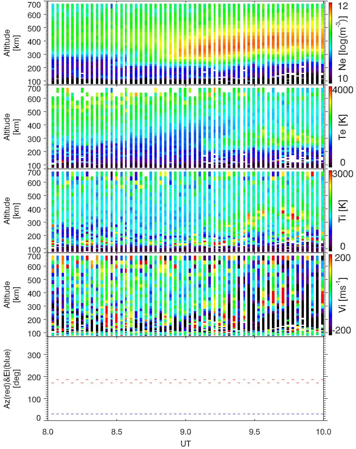
EISCAT 2001-12-12_08_10UT_tau0_ant@32m.
