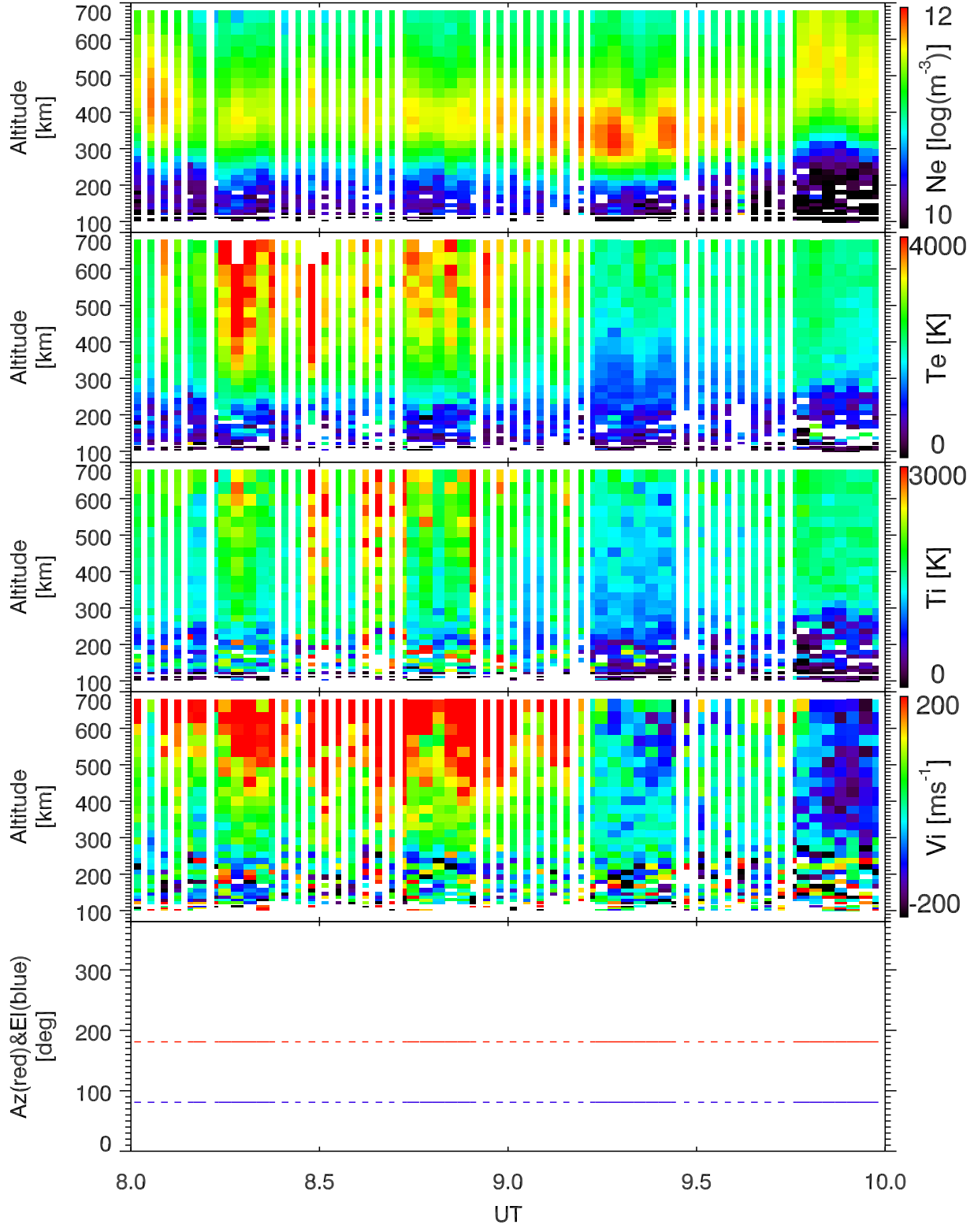
EISCAT 2001-12-12_08_10UT_tau0_120@42m.
