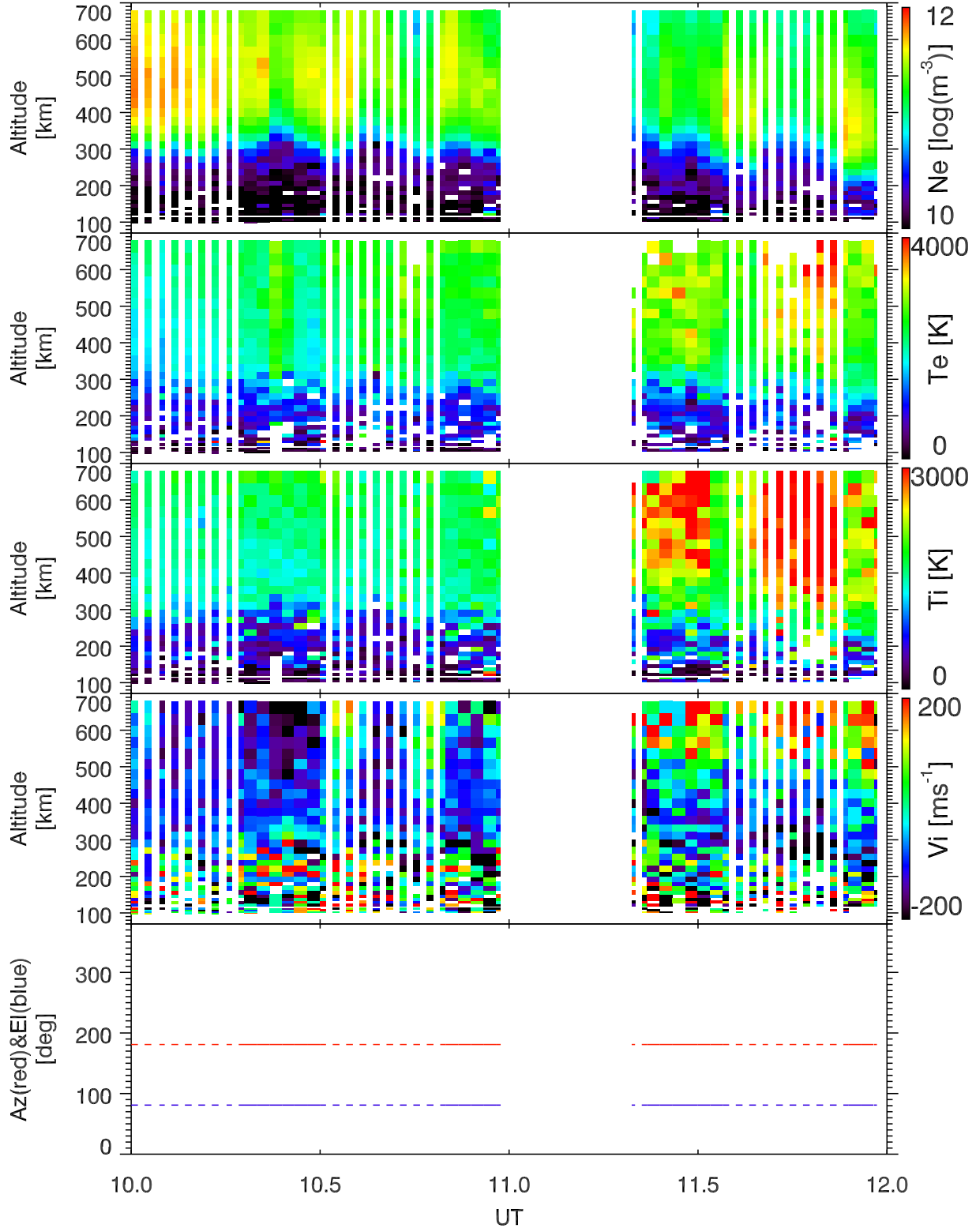
EISCAT 2001-12-12_10_12UT_tau0_120@42m.
