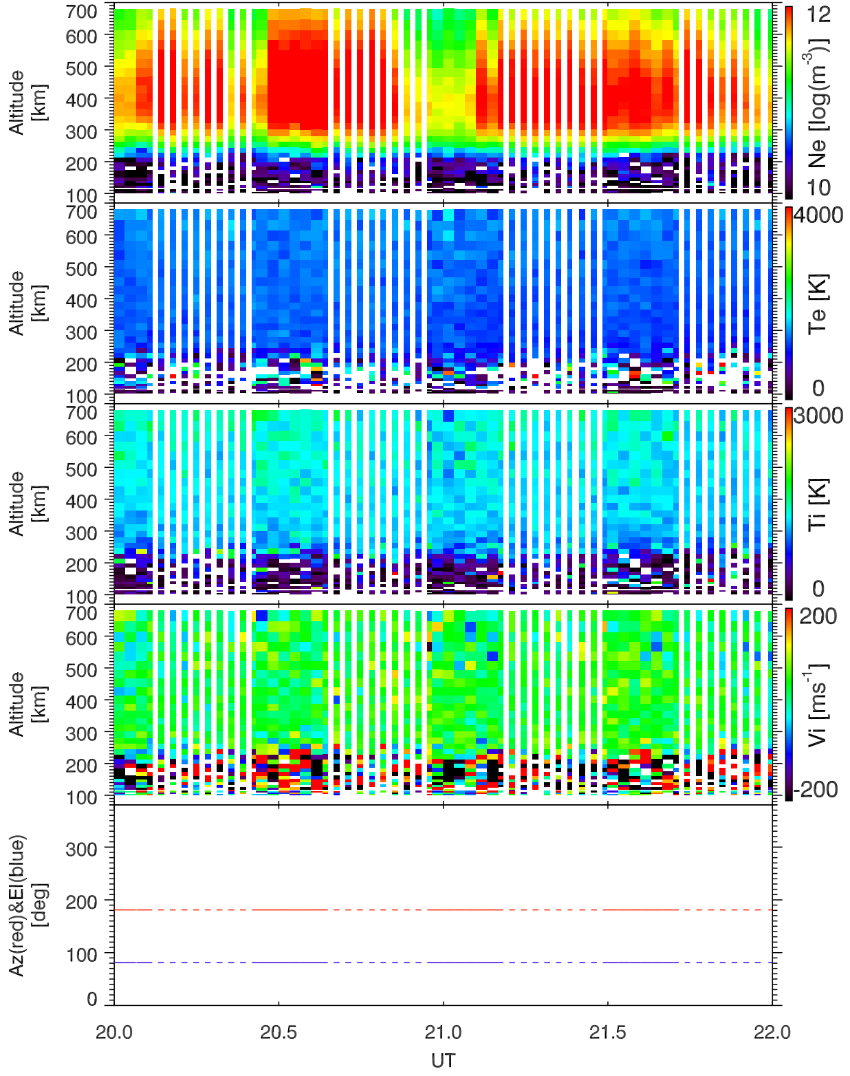
EISCAT 2001-12-12_20_22UT_tau0_120@42m.
