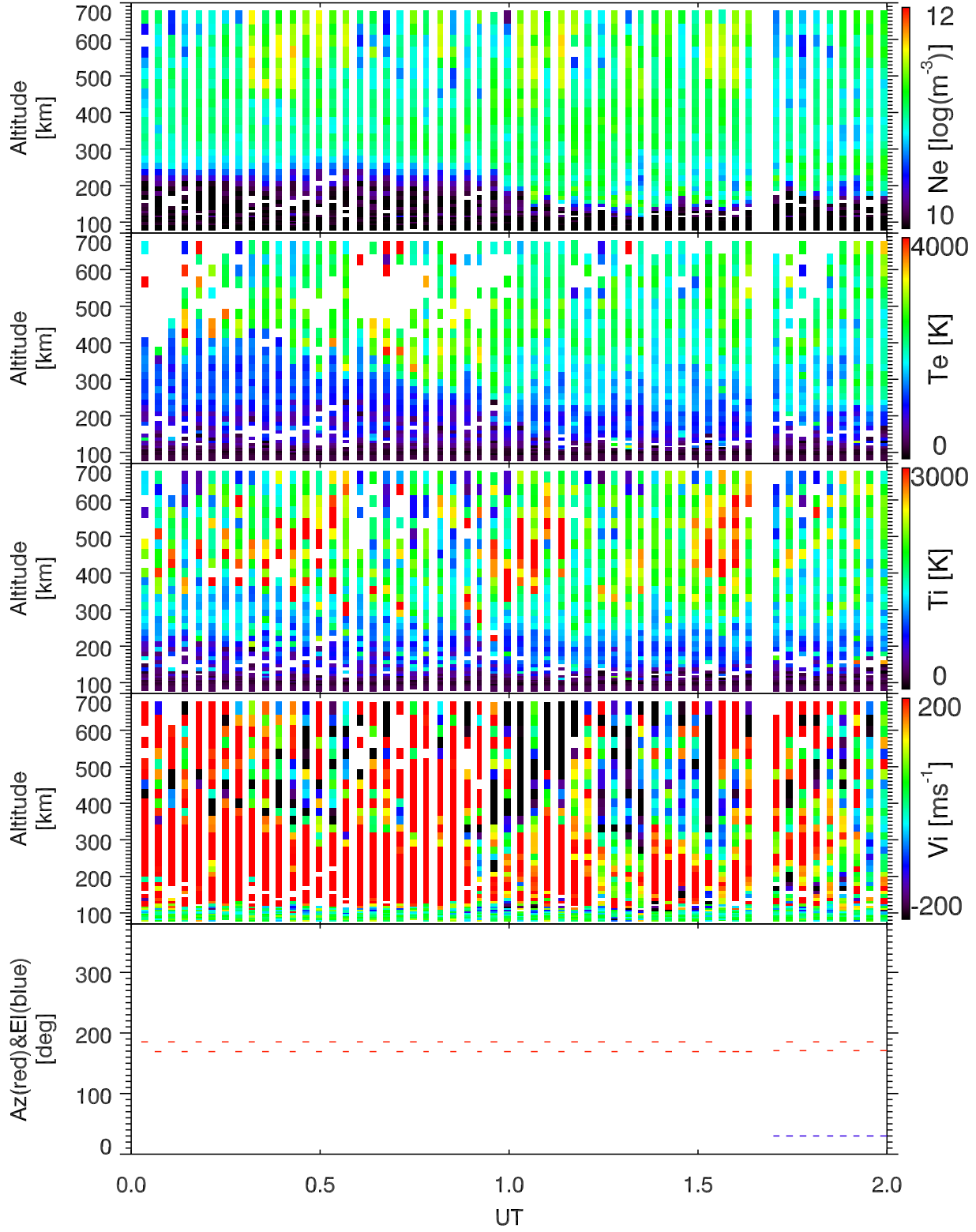
EISCAT 2001-12-13_00_02UT_tau0_ant@32m.
