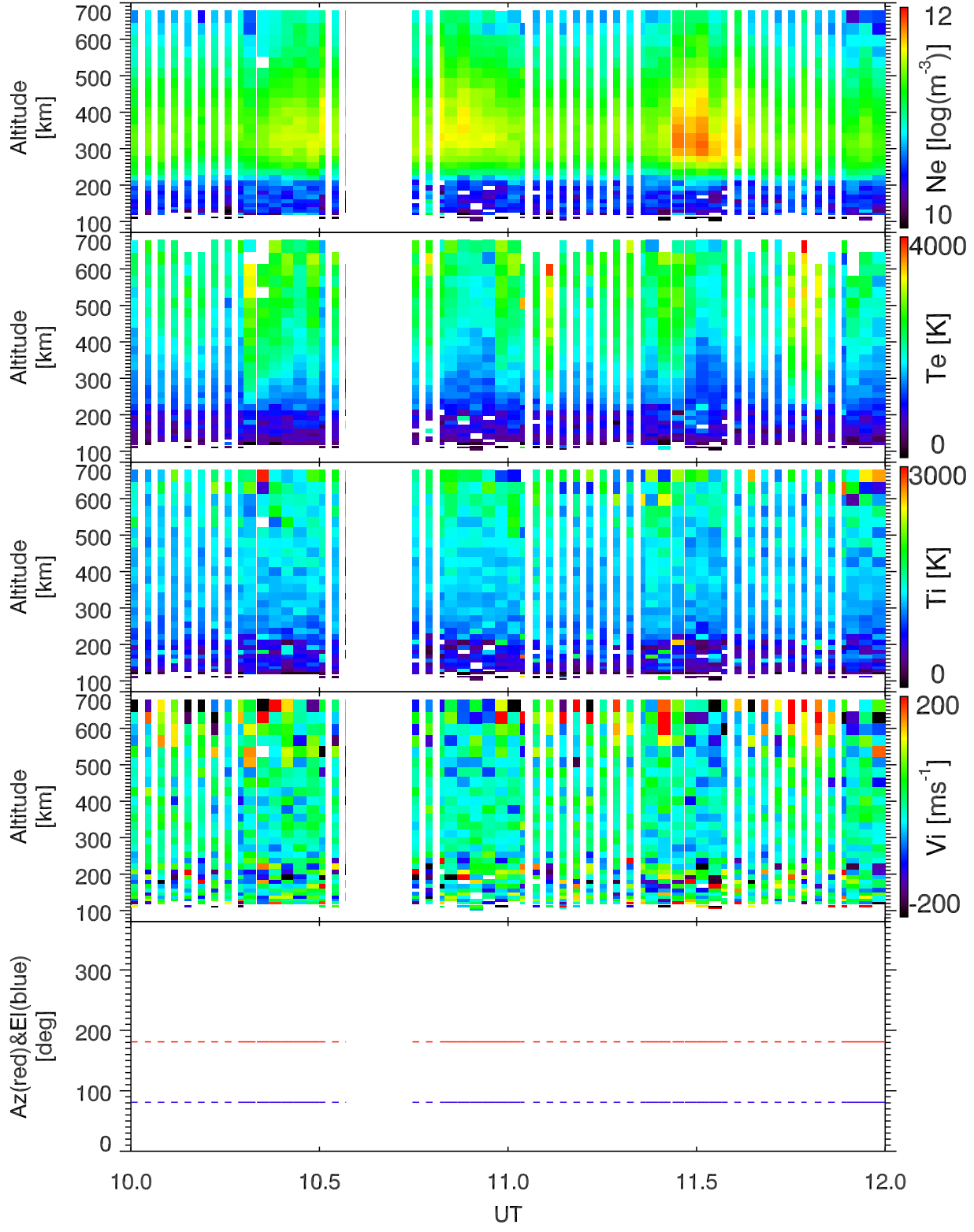
EISCAT 2001-12-13_10_12UT_tau0_120@42m.
