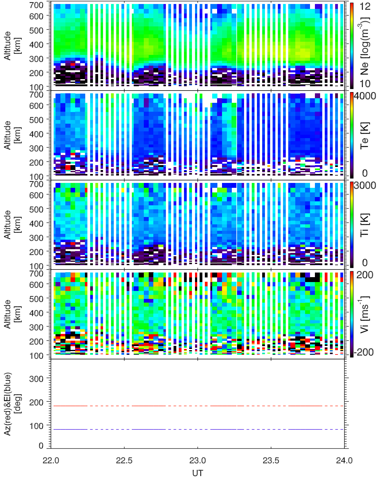
EISCAT 2001-12-13_22_24UT_tau0_120@42m.
