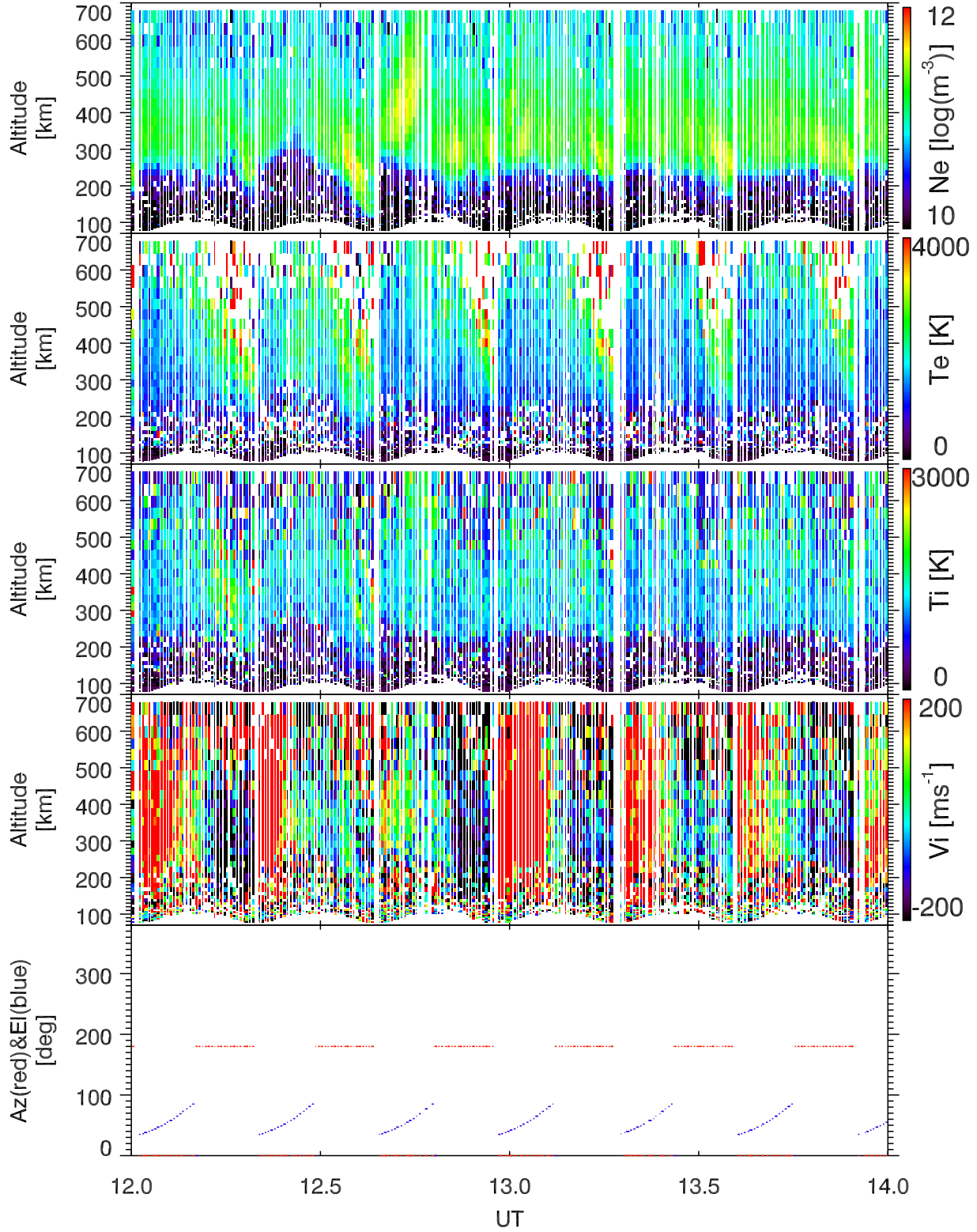
EISCAT 2001-12-18_12_14UT_tau0_all@32m.
