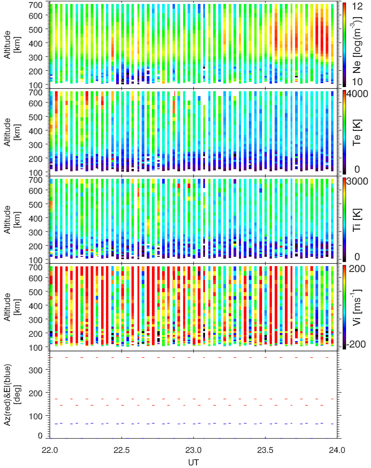
EISCAT 2002-01-20_22_24UT_tau0_all@32m.
