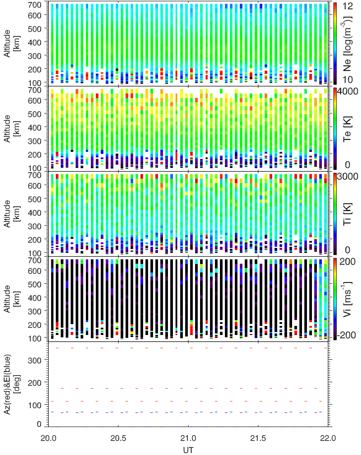
EISCAT 2002-07-28_20_22UT_tau0_ant@32m.
