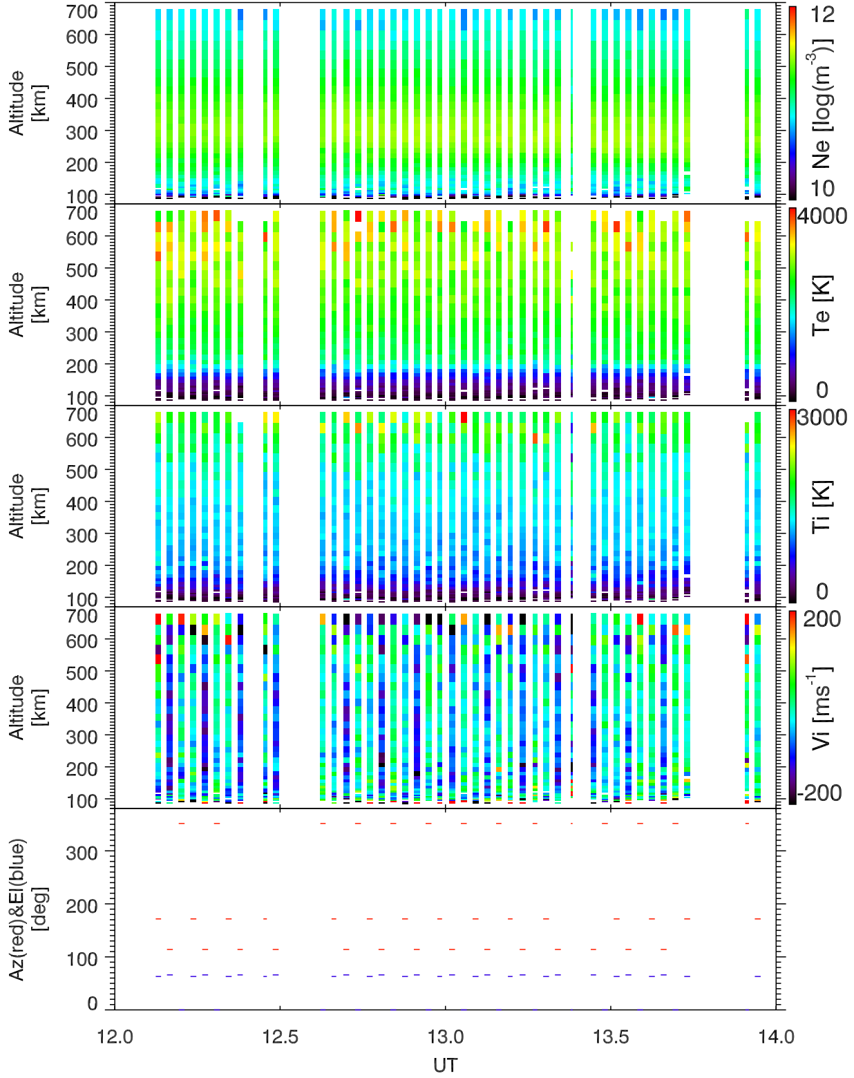
EISCAT 2002-08-06_12_14UT_tau0_ant@32m.
