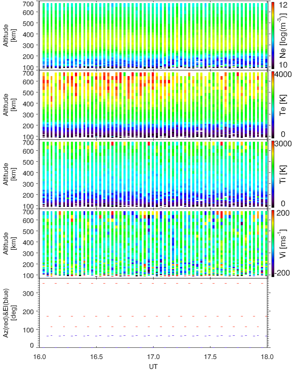
EISCAT 2002-09-01_16_18UT_tau0_ant@32m.
