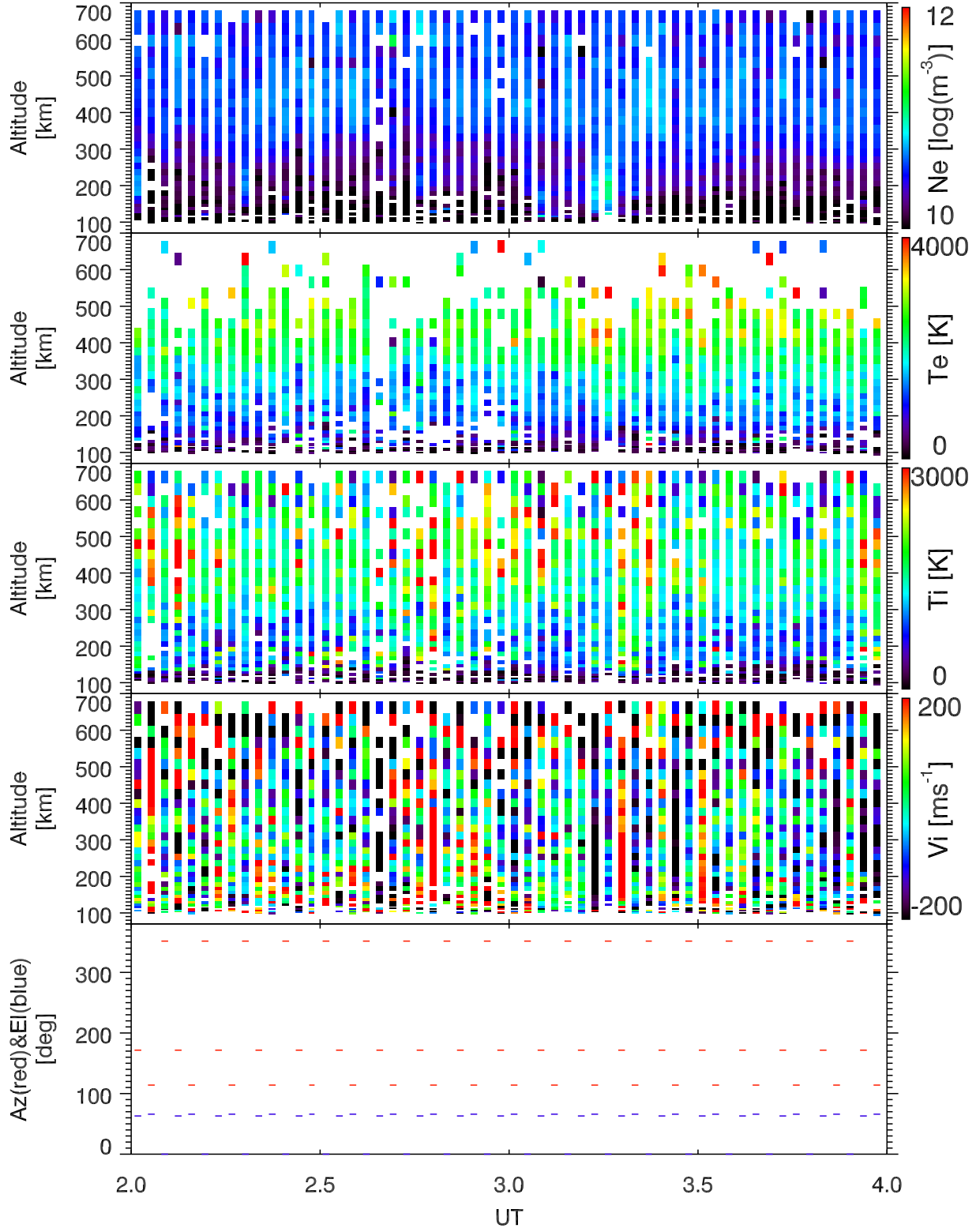
EISCAT 2002-10-05_02_04UT_tau0_ant@32m.
