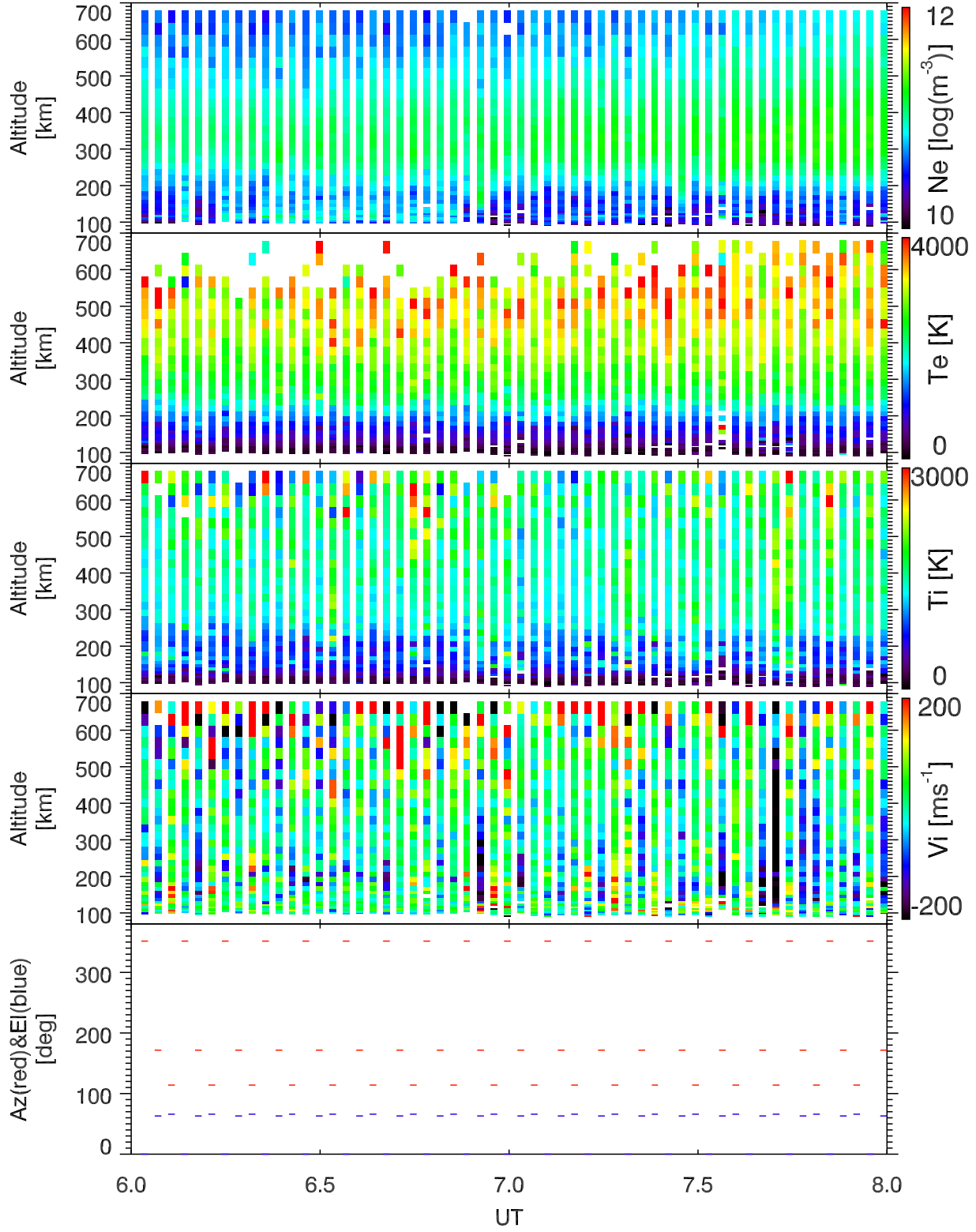
EISCAT 2002-10-05_06_08UT_tau0_ant@32m.
