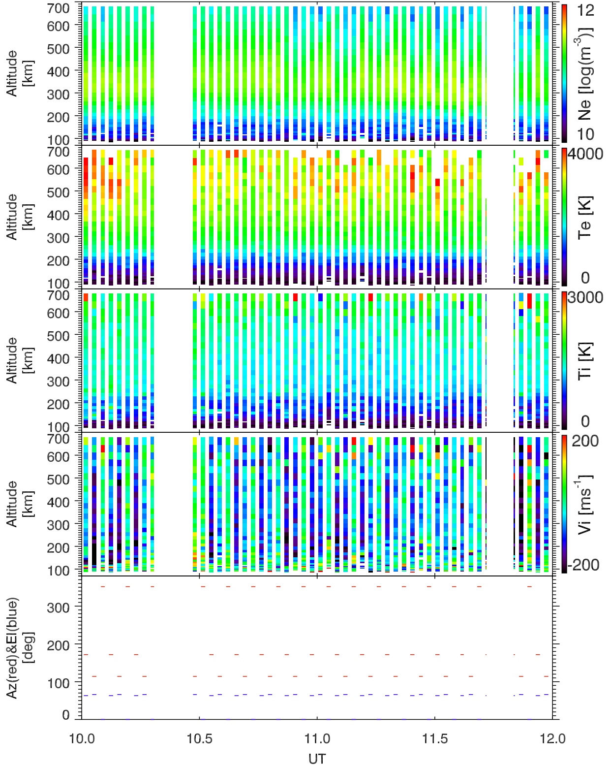
EISCAT 2002-10-05_10_12UT_tau0_ant@32m.
