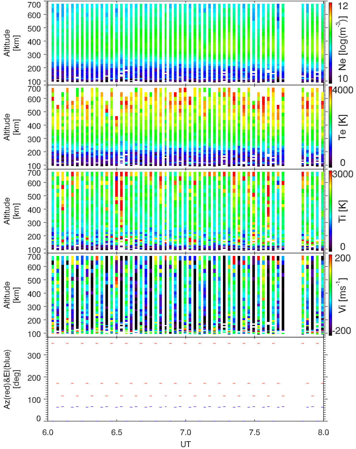
EISCAT 2002-10-06_06_08UT_tau0_ant@32m.
