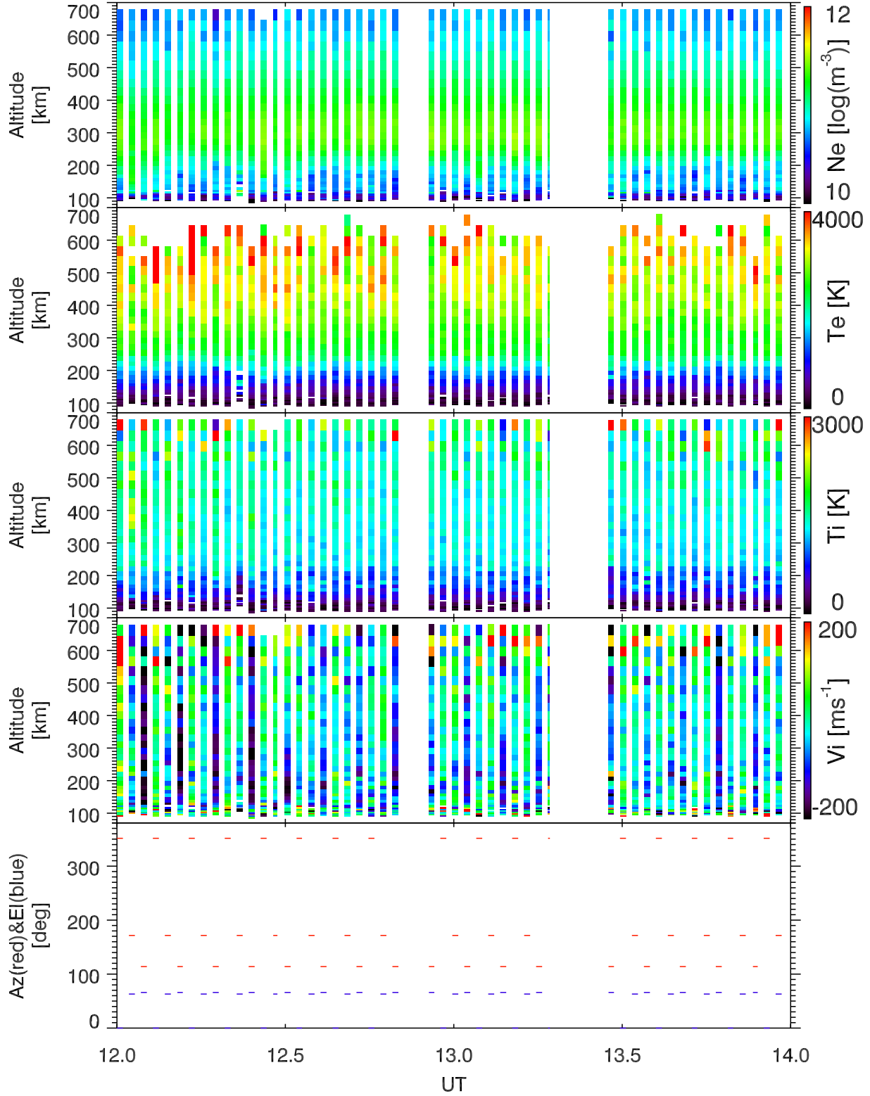
EISCAT 2002-10-06_12_14UT_tau0_ant@32m.
