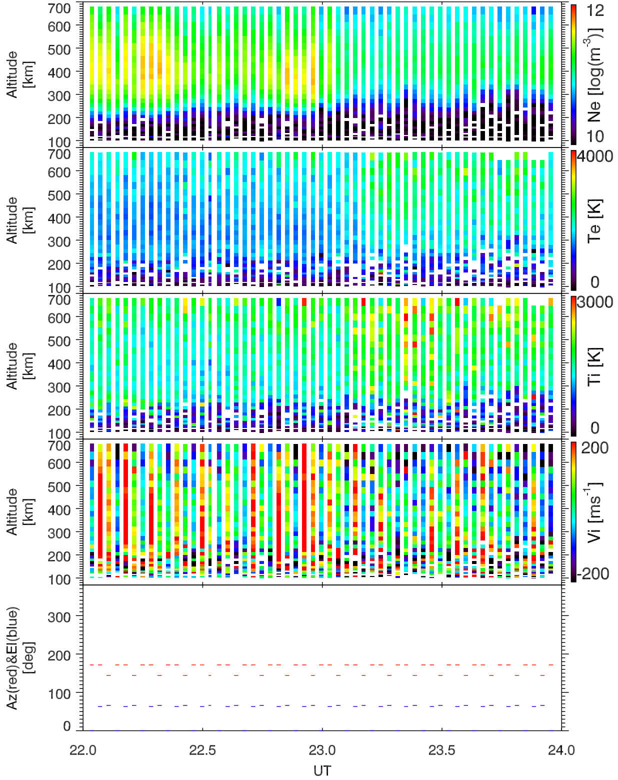
EISCAT 2002-10-06_22_24UT_tau0_ant@32m.
