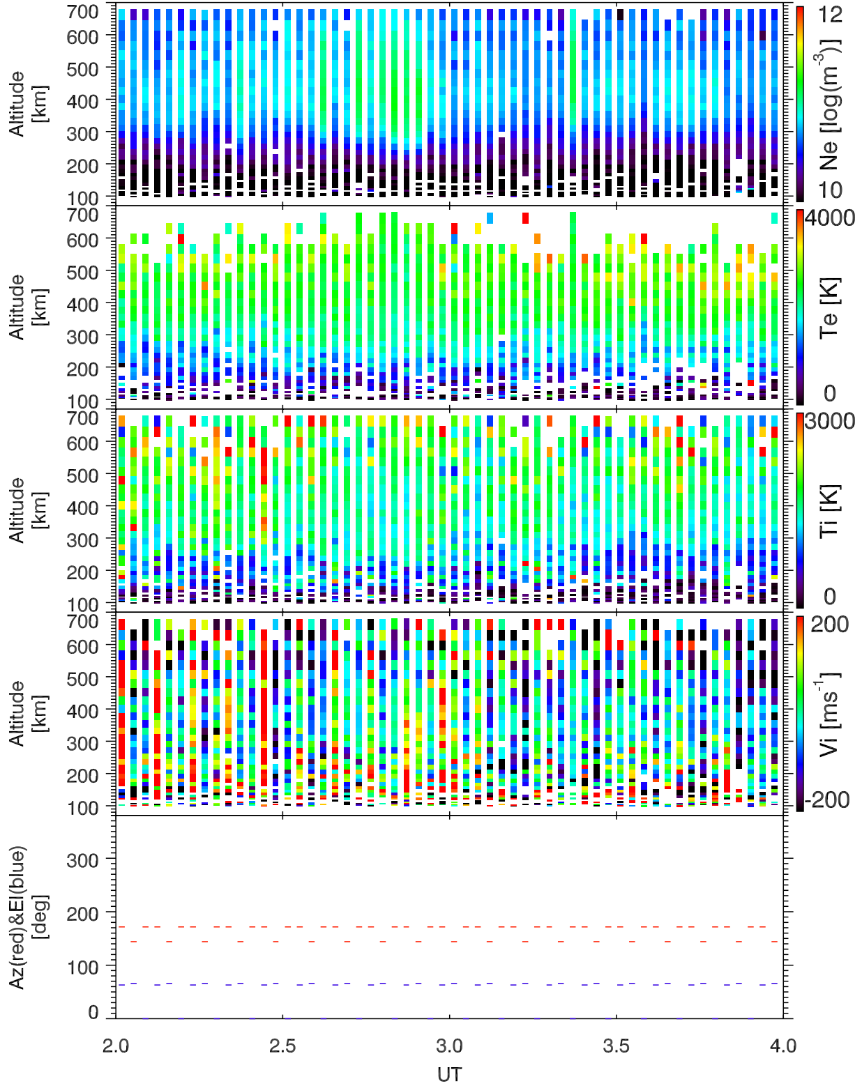
EISCAT 2002-10-07_02_04UT_tau0_ant@32m.
