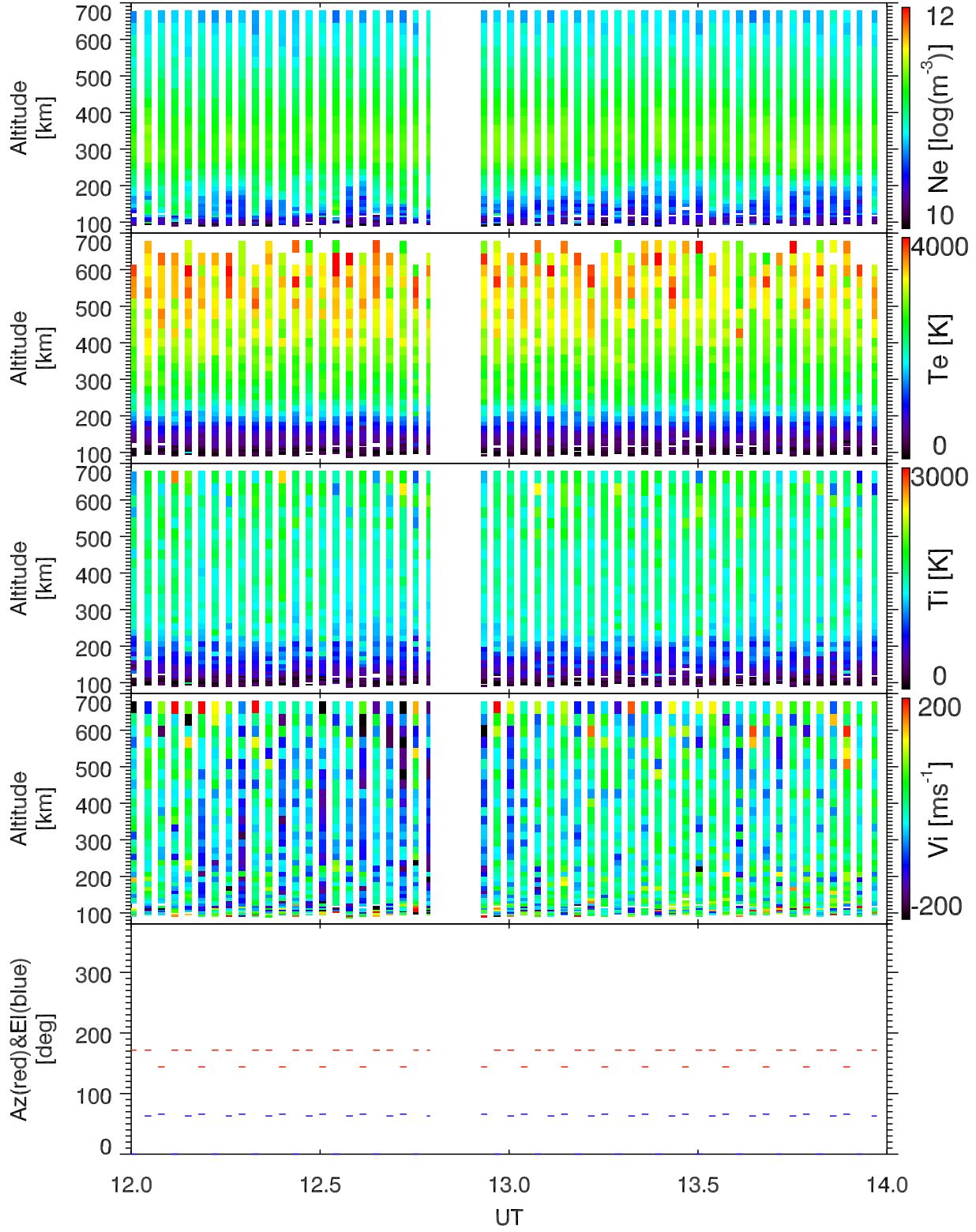
EISCAT 2002-10-08_12_14UT_tau0_ant@32m.
