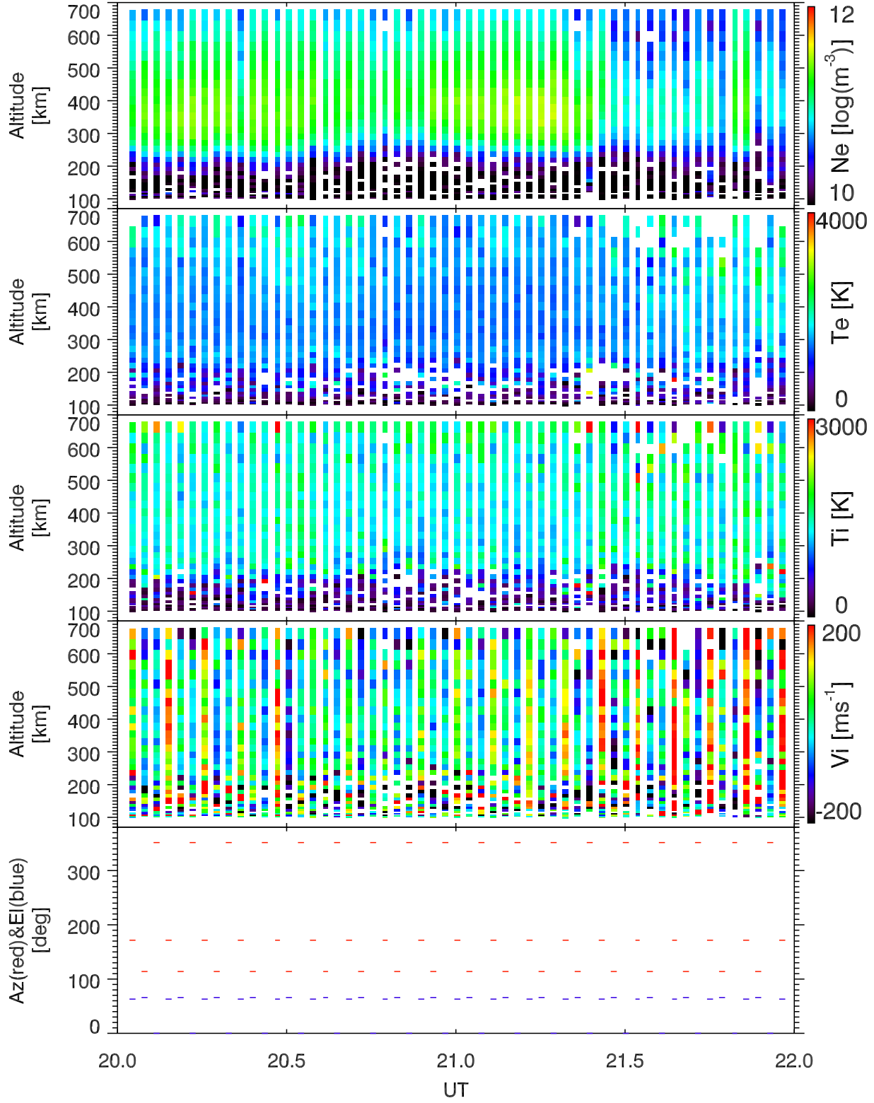
EISCAT 2002-10-08_20_22UT_tau0_ant@32m.
